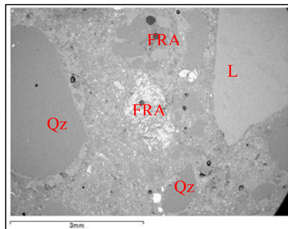
Figure 6. Comparison of the macro-positivity of concrete mixes with 100% FRA: detail of the interfacial transition zone of a FRA of a concrete mix made with 100% Ambilei's FRA (L—limestone, Qz—quartz). Bravo, M.; Santos Silva, A.; de Brito, J.; Evangelista, L. Microstructure of Concrete with Aggregates from Construction and Demolition Waste Recycling Plants, Microscopy and Microanalysis , 22, 149–167, reproduced with permission [10].
