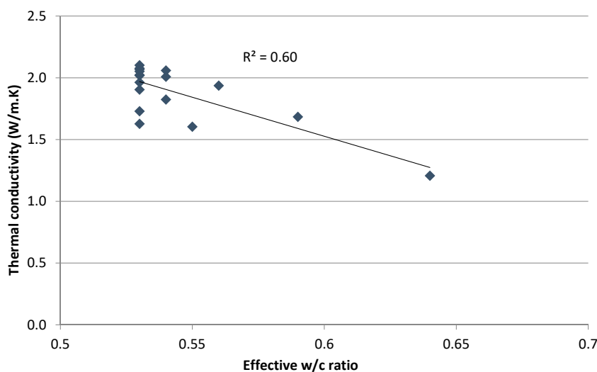
Figure 13. Variation of the thermal conductivity with the effective w/c ratio.
