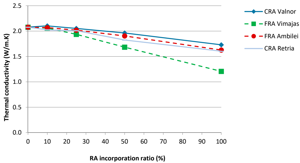
Figure 8. Thermal conductivity of the concrete mixes studied.
