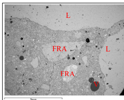
Figure 5. Comparison of the macro-porosity of concrete mixes with 100% FRA: detail of the interfacial transition zone of a FRA of a concrete mix made with 100% Vimajas’s FRA (L—limestone, V—voids). Bravo, M.; Santos Silva, A.; de Brito, J.; Evangelista, L., Microstructure of Concrete with Aggregates from Construction and Demolition Waste Recycling Plants, Microsc. Microanal. 22, 149–167, reproduced with permission [10].
