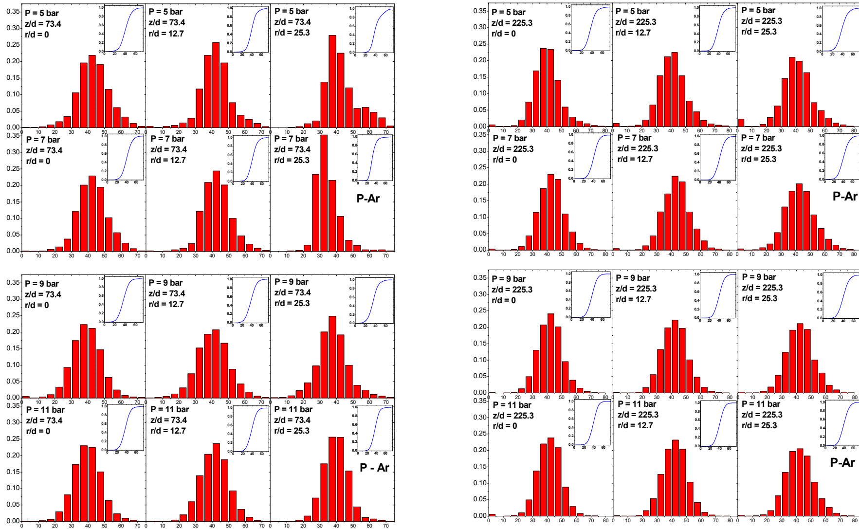
Figure S2. Droplet size distributions at three radial locations on the closest and the farthest measurement planes, for P-Ar blend.
