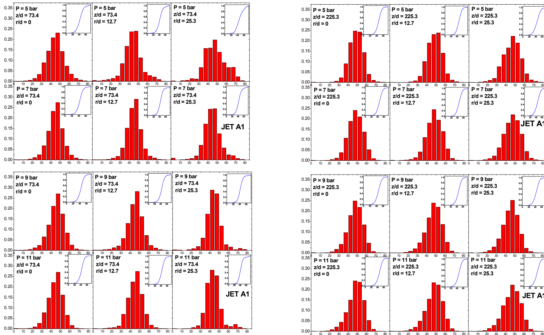
Figure S1. Droplet size distributions at three radial locations on the closest and the farthest measurement planes, for Jet A-1 fuel.
