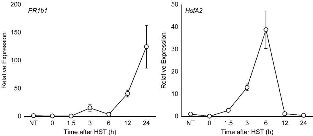
Figure S1. Changes in the relative expression level of (a) PR1b1 , and (b) HsfA2 . Gene expression levels in the first leaf at 0, 1.5, 3, 6, 12, or 24 h after HST (45 °C, 2 min), and NT were quantified by qPCR and normalized to GAPDH expression. Vertical bars indicate S. E. M. ( n = 4 ).
