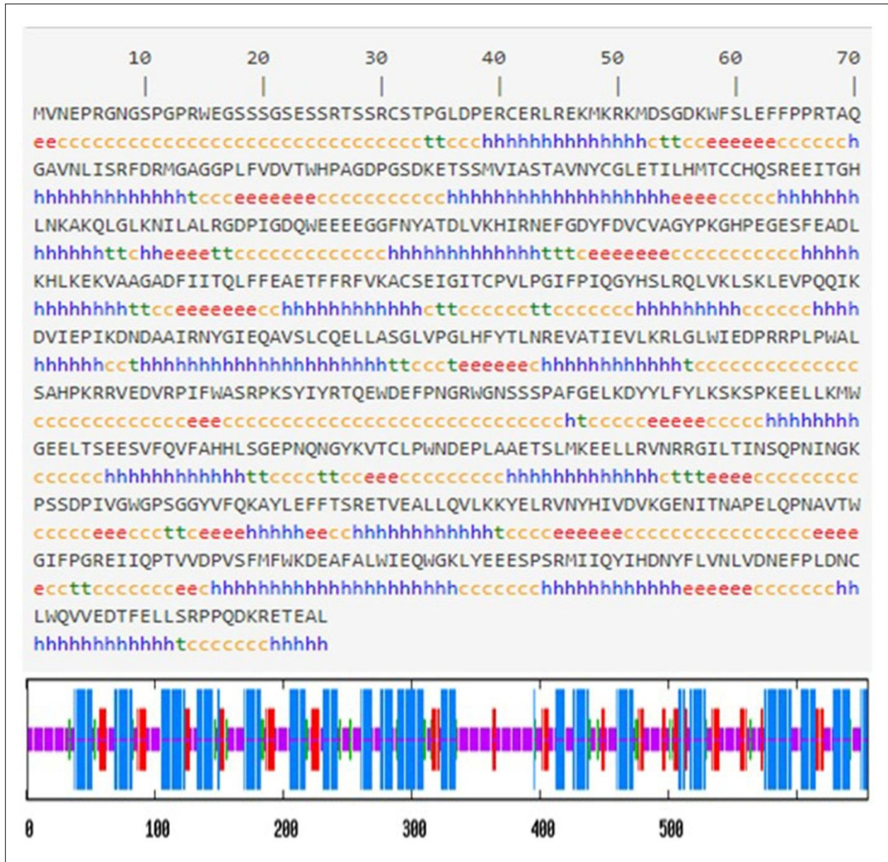
Figure S4. Predicted secondary structure of Bos taurus MTHFR. The long vertical zone: Alpha helix (h); The middle vertical zone: Extended strand (e); The short vertical zone: Random coil (c). The secondary structure was predicted by SOPMA online software.
