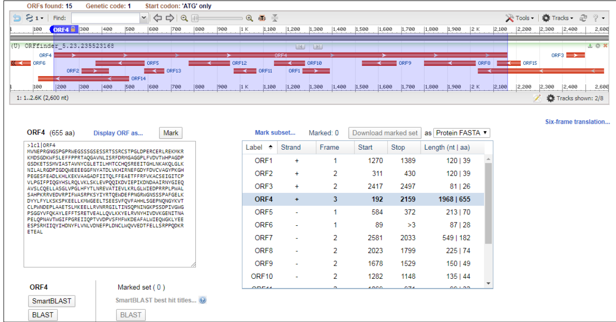
Figure S1. ORF analysis of yellow-cattle ( Bos taurus ) MTHFR sequence.
