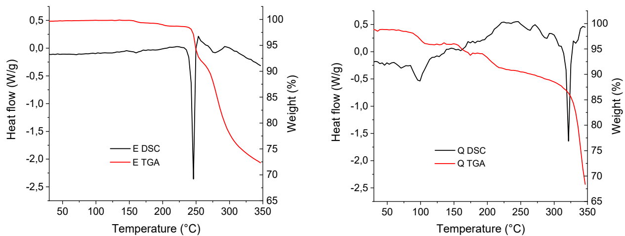
Figure 1. DSC y TGA curves for epicatechin (E) and quercetin (Q).
