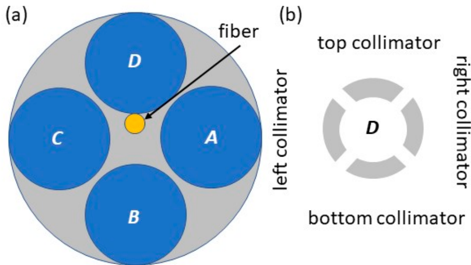
Figure 2. (a) Layout of the targets (blue) and fiber (yellow) in the inner position on the target selector (grey) looking upstream. Position A is housing a natural water target for the ^{16}\text{O}(p,a)^{13}\text{N} production, position B is a natural thallium target for the ^{203}\text{Tl}(p,n)^{203}\text{Pb} production, position C holds a target plug, and position D is an ^{18}\text{O}(p,n)^{18}\text{F} gas target. (b) Quadrant collimators in front of target port D looking upstream. Each target position has its own quadrant collimator.
