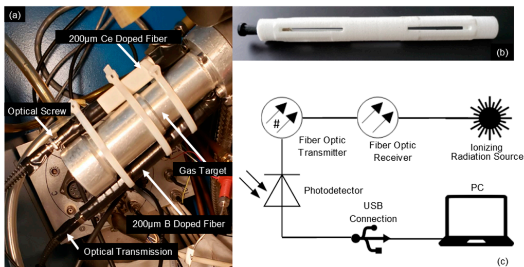
Figure 1. (a) 200 \mu\text{m} Ce-doped fiber and 200 \mu\text{m} B-doped fiber mounted to the ^{18}\text{F} gas target. (b) 200 \mu\text{m} borosilicate fiber in plastic housing without the black tape wrapping to prevent background from ambient light. (c) Schematic of the setup.
