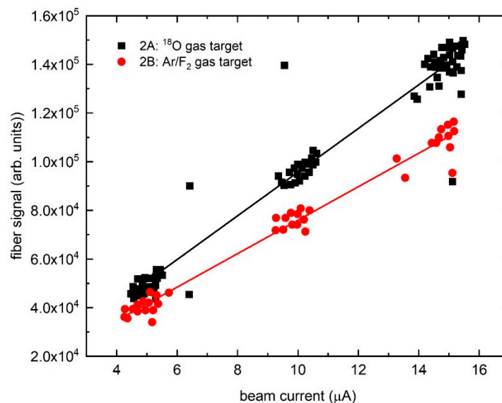
Figure 8. Graph comparing the difference in Ce-200 fiber signal between the irradiation of ^{18}\text{O} gas and \text{Ar}/\text{F}_2 mixture. The adjusted R^2 values are 0.9838 and 0.9945, respectively.
