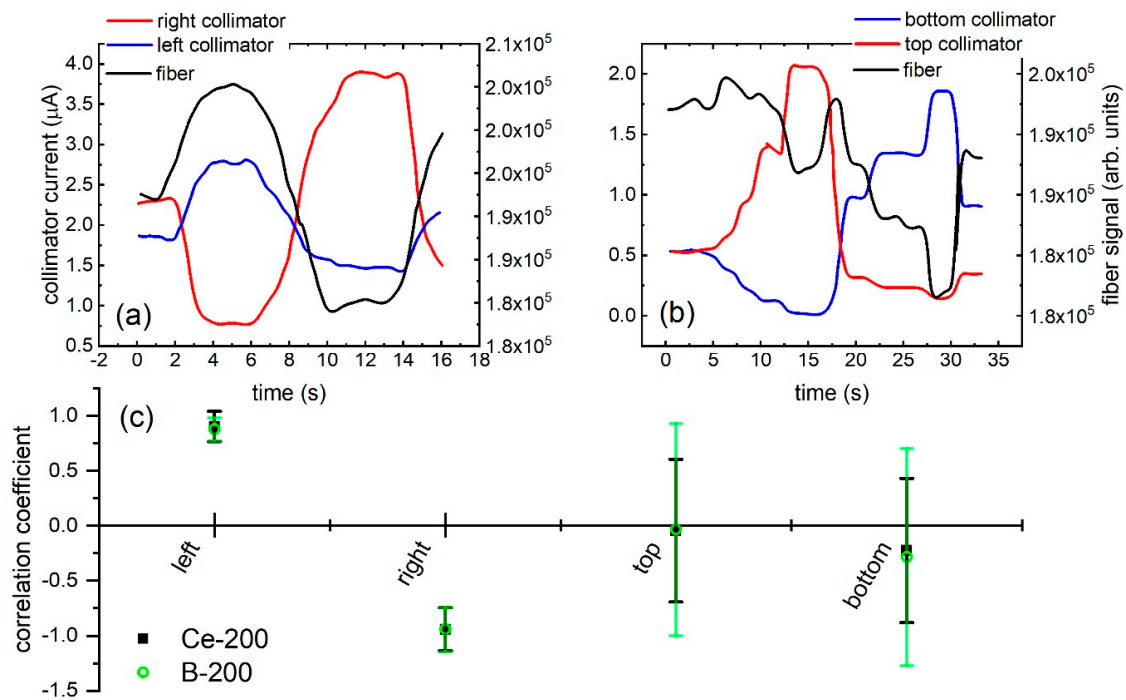
Figure 4. In (a,b), the collimator currents are compared with the Ce-200 fiber’s signal while at a beam current on the target of 20 \mu A. Both fibers are mounted at the side of the target closest to the bottom collimator. The bar graph in (c) expresses the correlations between the collimator currents and the fiber signal when the target selector was moved in the plane that the collimators were positioned in, and the beam current’s correlation during these periods.
