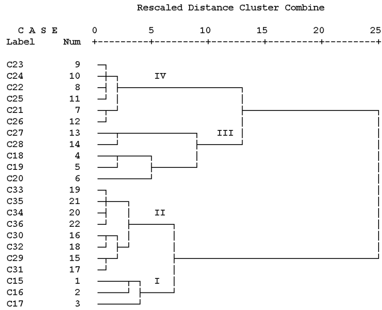
Dendrogram using Average Linkage For n-FAs (Between Groups)
