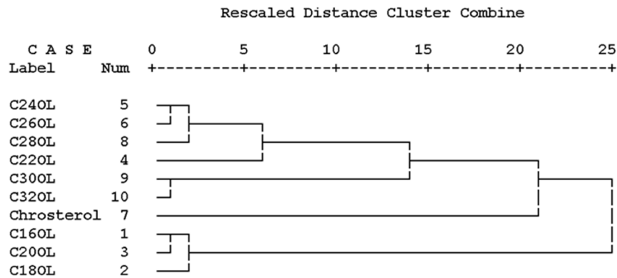
Dendrogram using Average Linkage for Alkanols (Between Groups)
