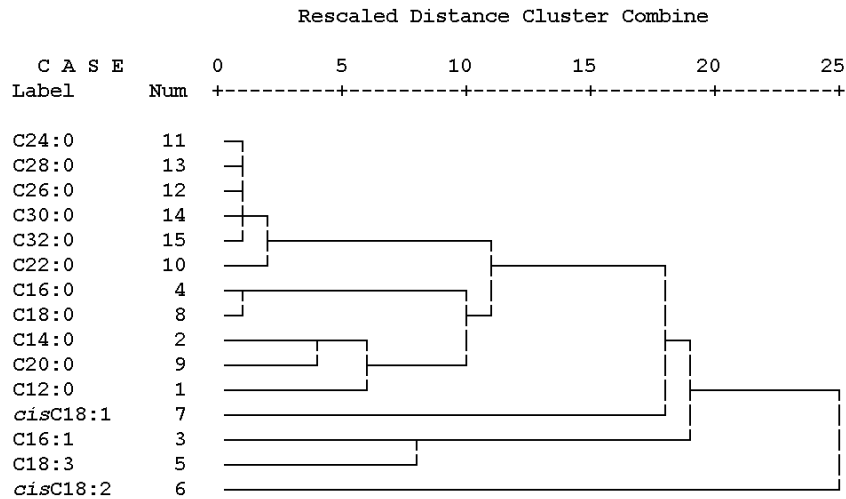
Dendrogram using Average Linkage For n-FAs (Between Groups)
