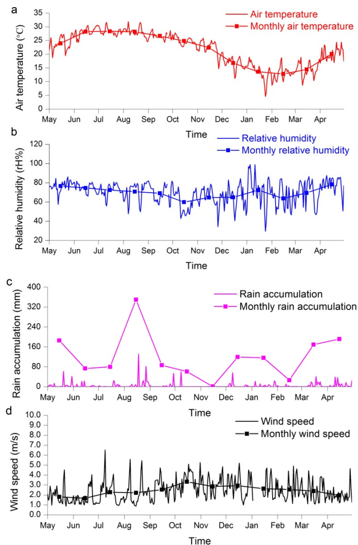
Figure S1. Daily and monthly meteorological characteristics in Xiamen during the period from 1 May 2015 to 30 April 2016. (a) air temperature; (b) relative humidity; (c) rain accumulation; and (d) wind speed.
