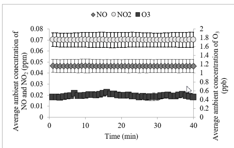
Figure S1. The ambient pollution concentration profiles within the flow reactor procedural control treatments (data are means, n = 14 , errors bars represent the SEM).
