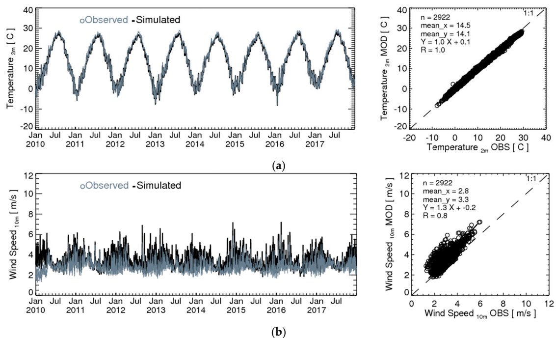
Figure 2. Comparisons of observed and simulated daily mean values of (a) 2-m temperatures and (b) 10-m wind speeds. These values were spatially averaged over 98 METeoro logical Aerodrome Reports (METAR) sites in South Korea and China.
