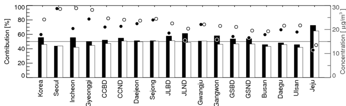
Figure 7. The eight-year average PM 2.5 concentrations (circles) and the Chinese contribution (bars) in the 17 provinces via the 9-km simulation. The black and white colors represent the area-based and monitor location-based Chinese contribution, respectively.
