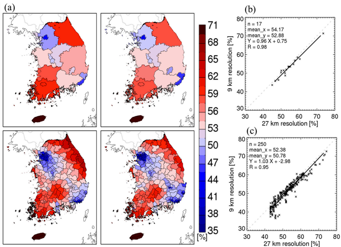
Figure 5. The eight-year mean Chinese contribution to PM_{2.5} concentrations in 17 provinces ( a-top ) and 250 prefectures ( a-bottom ) in South Korea estimated via the 27- ( a-left ) and 9-km ( a-right ) simulations from 2010 to 2017. Scatter plots of the Chinese contribution estimated via the 27- and 9-km simulations for (b) the 17 provinces and (c) the 250 prefectures.
