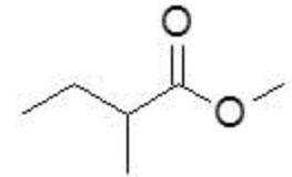
methyl 2-methylbutanoate
