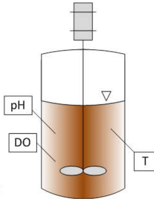
Biotransformation
