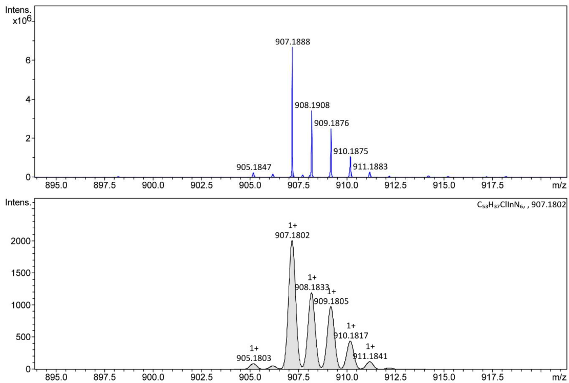
Figure 5. HR-MS spectrum of 1In.
