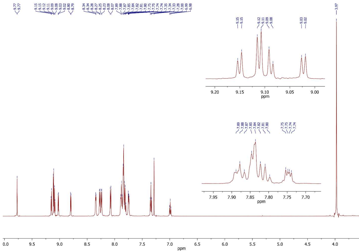
Figure 2. NMR spectrum of 1In in \text{CDCl}_3 .
