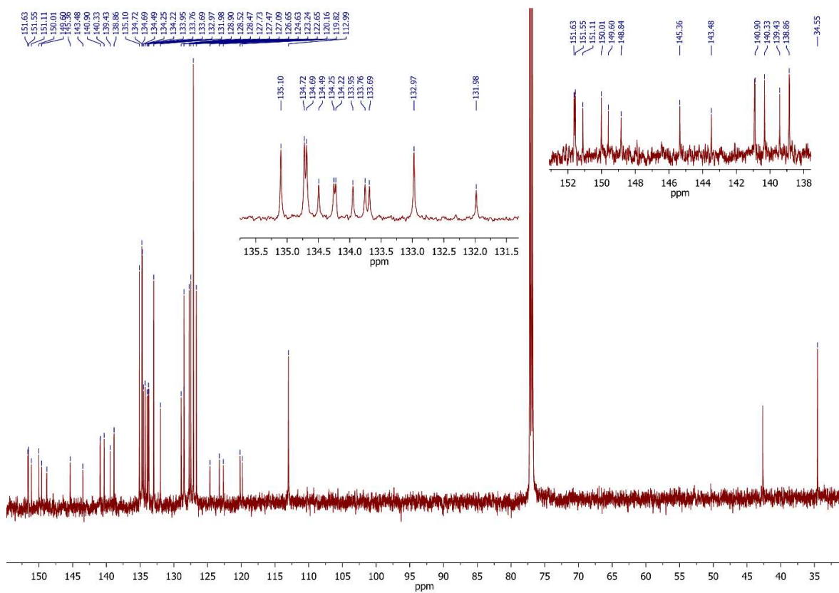
Figure 3. ^{13}\text{C} NMR spectrum of 1In in \text{CDCl}_3 .
