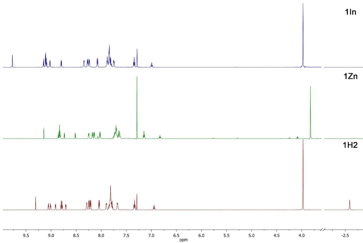
Figure 1. ^1\text{H} NMR spectra of 1H2 and 1In in \text{CDCl}_3 . ^1\text{H} NMR spectrum of 1Zn was recorded in \text{CDCl}_3/\text{MeOD} mixture (1/1) in the presence of 2 equiv. DABCO.
