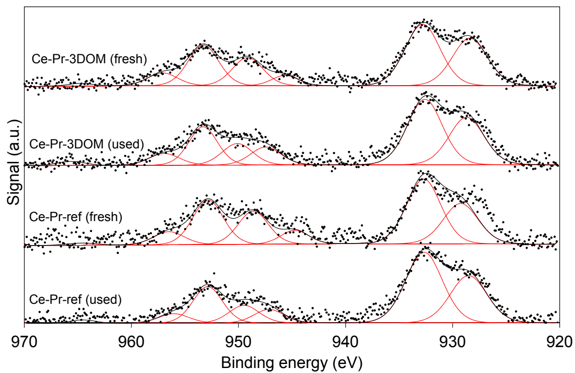
Figure S2. X-ray photoelectron spectra in the energy range of Pr 3d.
