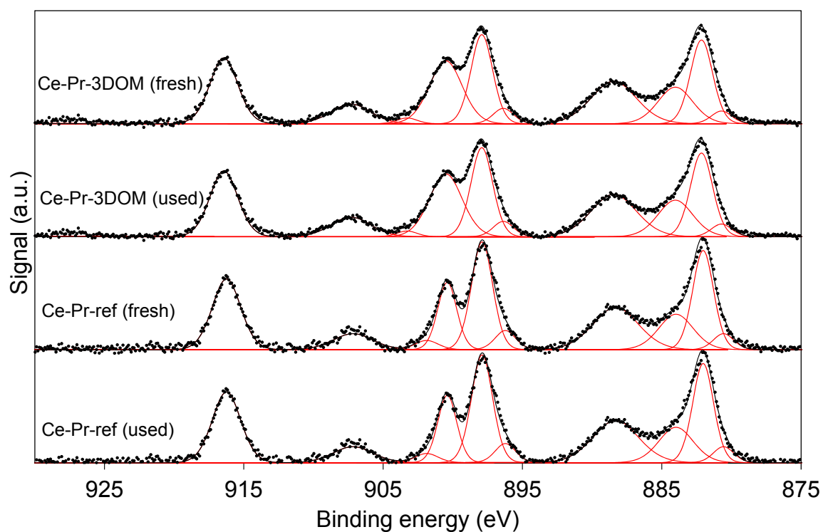
Figure S1. X-ray photoelectron spectra in the energy range of Ce 3d.
