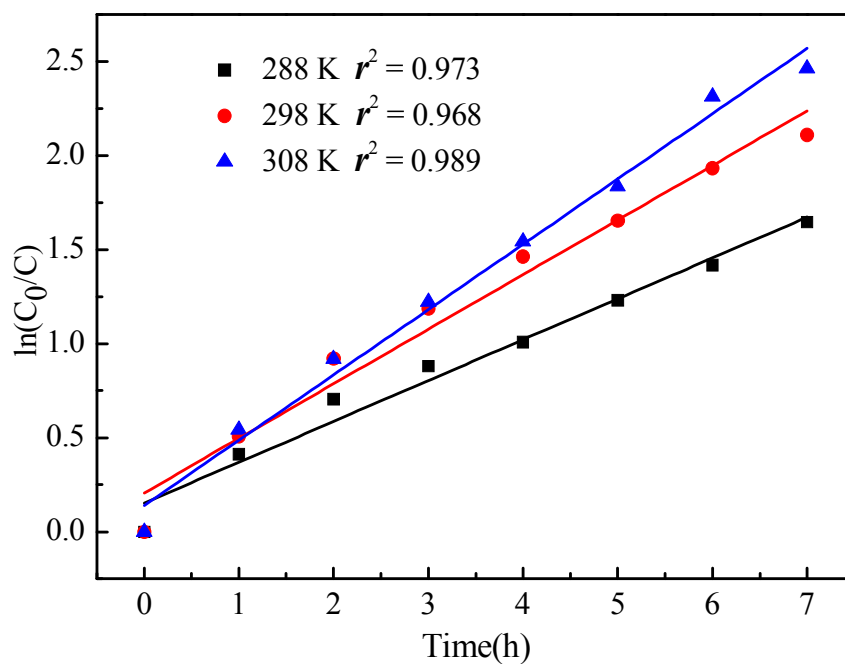
Figure S3. Pseudo-first-order kinetics degradation for RhB by ZnCr-0.75SalenCo-LDHs at different temperatures.
