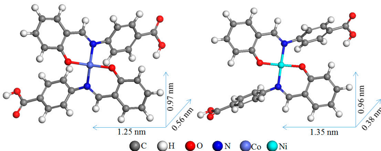
Figure S2. The structures of Salen-Co and Salen-Ni.
