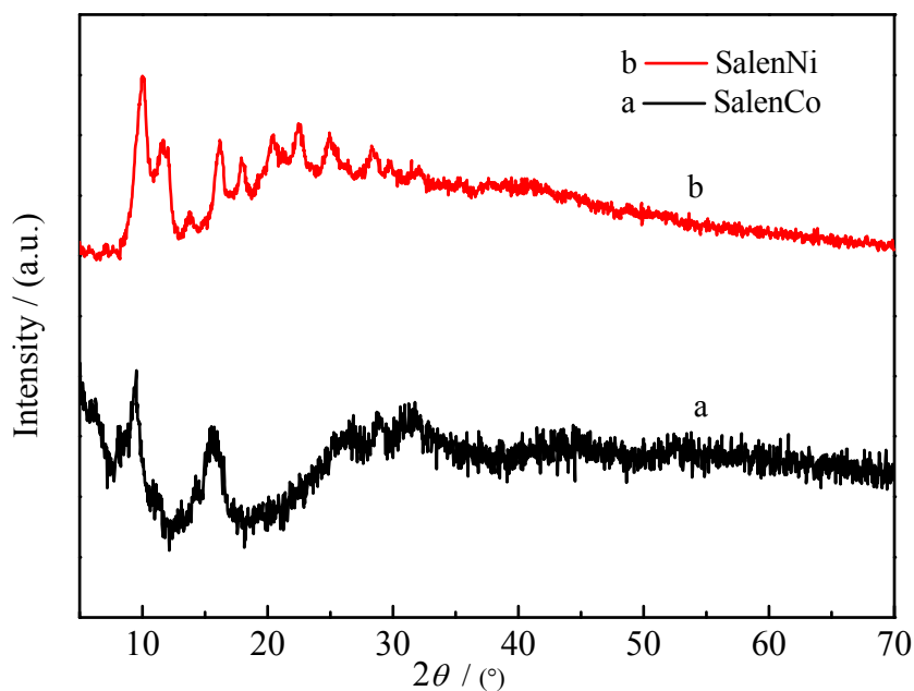
Figure S1. XRD patterns of SalenM.
