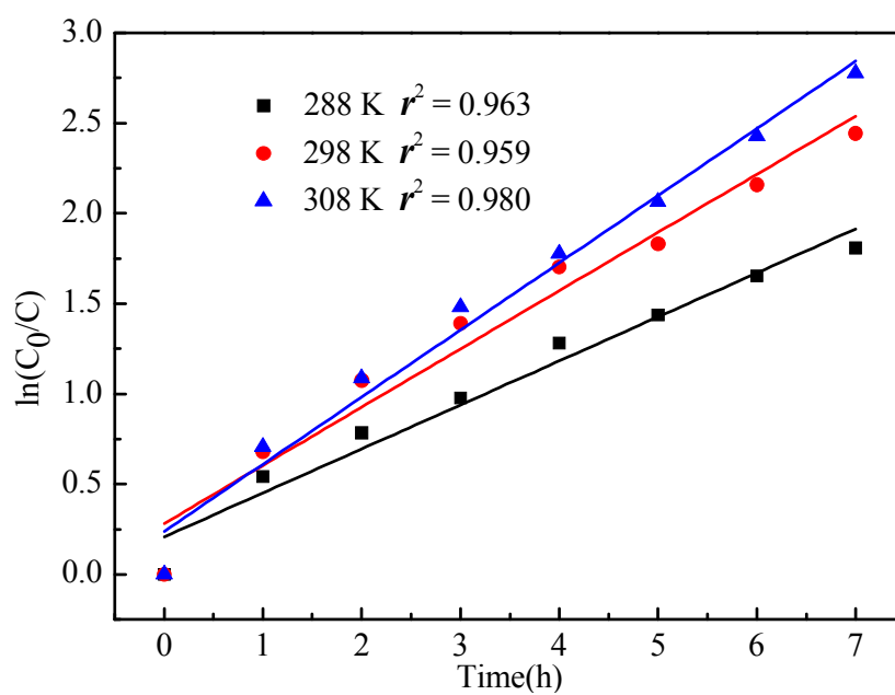
Figure S4. Pseudo-first-order kinetics degradation for RhB by ZnCr-0.75SalenNi-LDHs at different temperatures.
