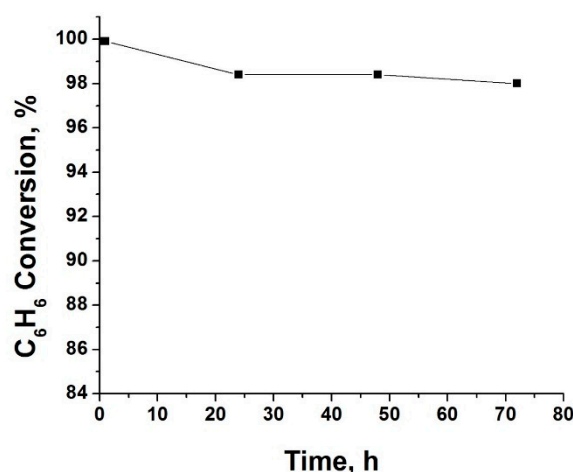
Figure S1. Stability test of Pd–AuYCeIM catalyst performed for 72 h at 150 °C.
