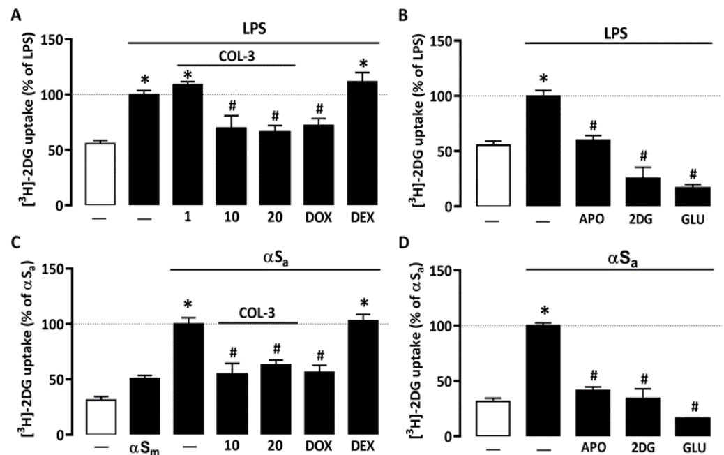
Figure 3. COL-3 reduces glucose accumulation in microglial cells exposed to either LPS or \alpha\text{Sa} . (A) Quantification of glucose uptake in microglial cells exposed or not to LPS (10 ng/mL, 24 h) in the presence or absence of COL-3 (10 or 20 \mu\text{M} ), DOX (50 \mu\text{M} ), or DEX (2.5 \mu\text{M} ). (B) Quantification of glucose uptake in microglial cells exposed or not to LPS treatment in the presence or absence of APO (300 \mu\text{M} ) or 2-DG (500 \mu\text{M} ). The specificity of the assay was confirmed by acutely exposing LPS-treated cell cultures to an excess of glucose (50 mM). (C) Quantification of glucose uptake in microglial cells exposed or not to \alpha\text{Sa} (70 \mu\text{g}/\text{mL} , 24 h) in the presence or absence of COL-3 (10 and 20 \mu\text{M} ), DOX (50 \mu\text{M} ), or DEX (2.5 \mu\text{M} ). (D) Quantification of glucose uptake in microglial cells exposed or not to \alpha\text{Sa} in the presence or absence of APO (300 \mu\text{M} ) or 2-DG (500 \mu\text{M} ). The specificity of the assay was confirmed by acutely exposing \alpha\text{Sa} -treated cell cultures to an excess of glucose (50 mM). Data are the mean \pm SEM ( n = 6\text{--}8 ). * p < 0.05 vs. control; # p < 0.05 vs. corresponding inflammogen. One-way ANOVA followed by Bonferroni post-hoc test.
