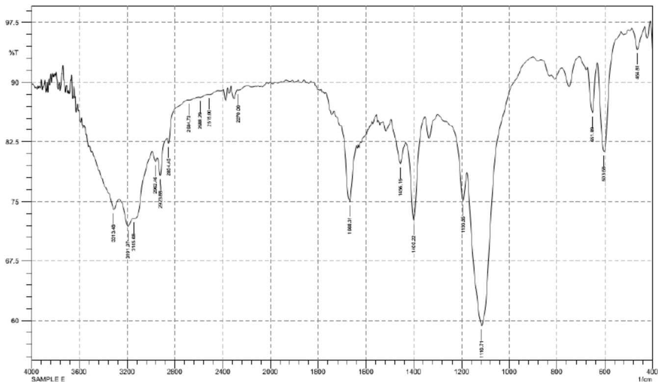
Figure 1. FT-IR spectrum of Ethyl acetate extract.
