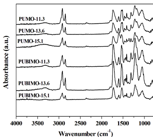
Figure S1. FTIR spectra of PUMO-11.3, PUMO-13.6, PUMO-15.1, PUBIMO-11.3, PUBIMO-13.6, and PUBIMO-15.1.
