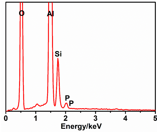
Figure S1. The EDS spectrum of PEO coating formed at 60 min.
