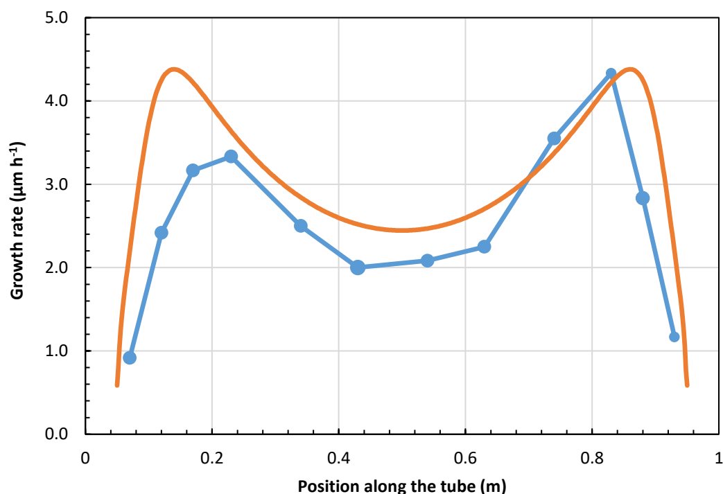
Figure 9. Calculated (–) and experimental (●) growth rate of \text{CrC}_x coatings along the inner wall of the tube reactor 1 m long with the injection of the precursor successively and alternately at each end ( T = 400\text{ }^\circ\text{C} ; P = 1.3 \times 10^3\text{ Pa} ; duration = 2 \times 3\text{ h} ; 500 sccm \text{N}_2 ; injection of 0.5\text{ g min}^{-1} of precursor solution in toluene containing 10.3 wt. % of bis(ethylbenzene)chromium (BEBC)).
