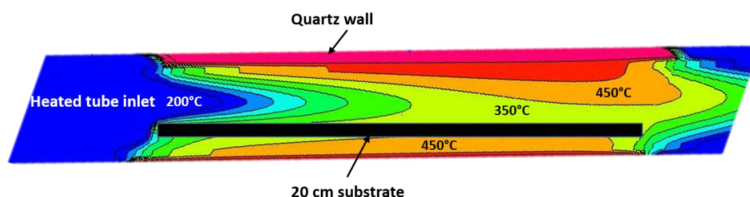
Figure 5. Temperature field in the central X–Y slice of the tubular reactor schematized in Figure 1b (Table 4, Run 1).
