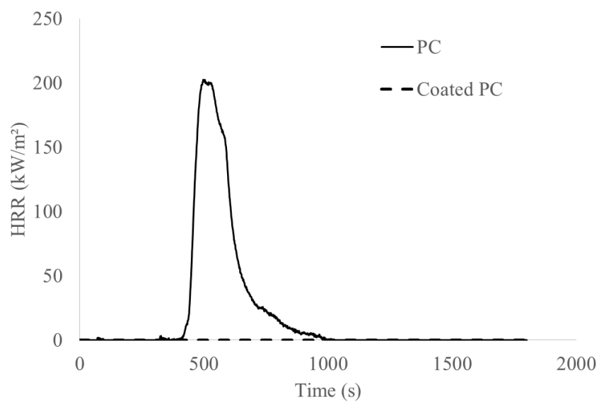
Figure S1. HRR curves obtained with PC and coated PC with the self-stratified epoxy/silicone compositions containing RDP and BDP FR additives at 2.5 wt.% and 5 wt.% (the four curves overlapped).
