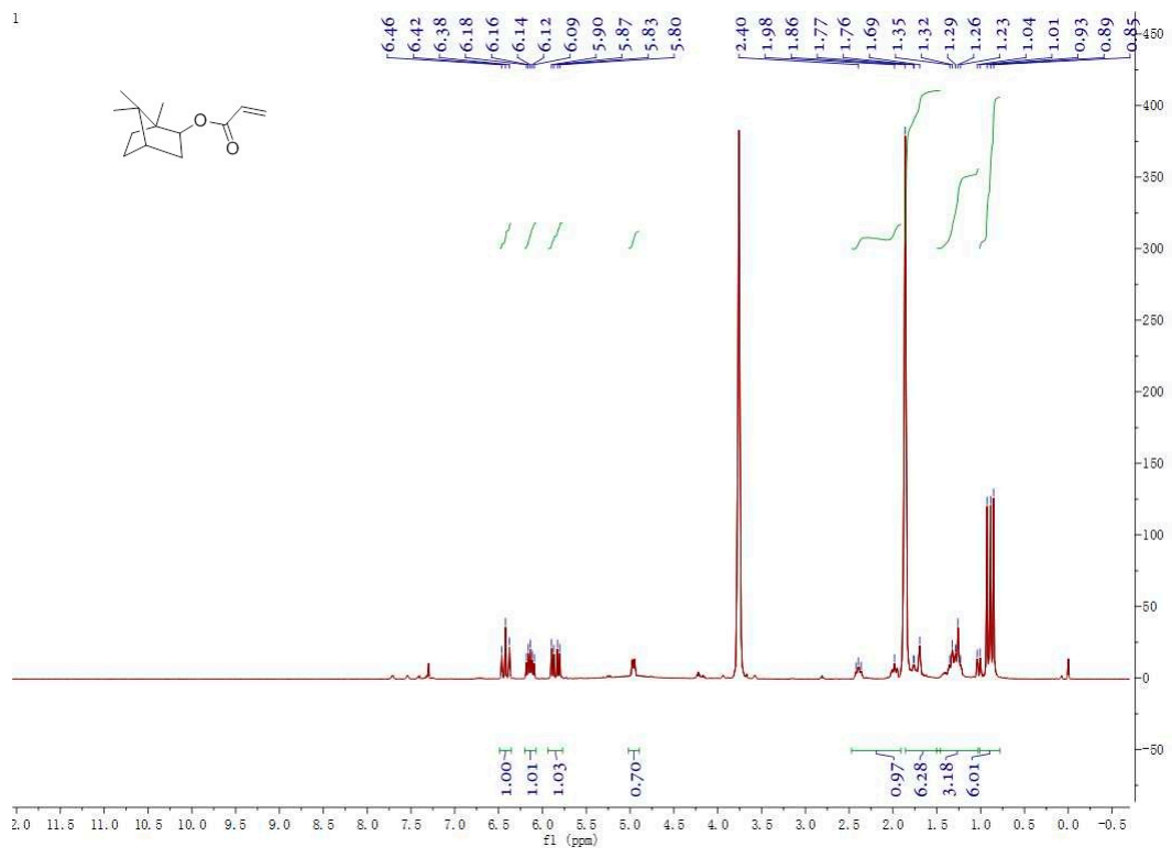
Figure S1. The 1 H NMR spectra of the BA.
