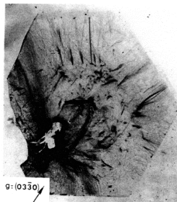
Figure 2. Dislocations in \alpha - \text{Al}_2\text{O}_3 crystal.
