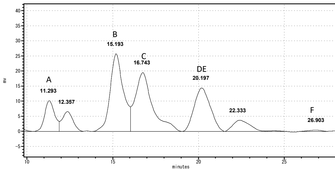
Figure S1 Typical surfactin standard chromatogram in HPLC showing surfactin isoform A-F.
