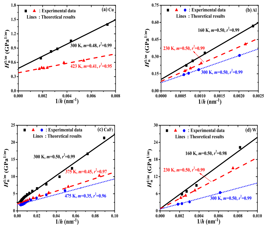
Figure 2. (Color online) Comparison of the H_n^{1/m}-1/h relationships at various temperatures between theoretical results (lines) and experimental data (dots) for (a) Cu [24], (b) Al [16], (c) CaF 2 [25] and (d) W [16].
