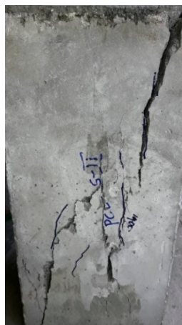
(i) Control PC column
