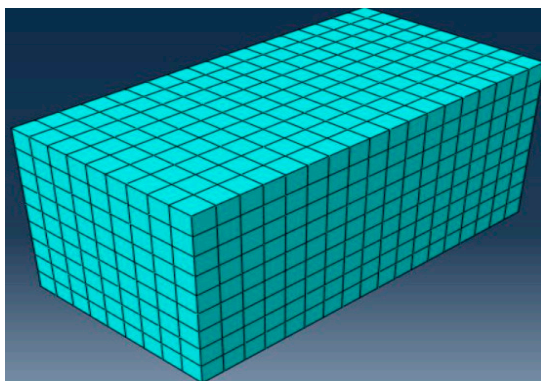
(i) C3D8R element—Concrete
