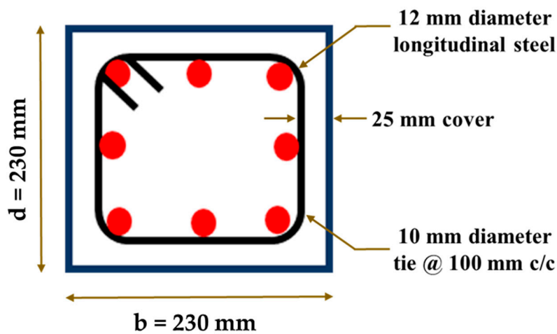
Figure 1. Sectional details of RC column elements.
