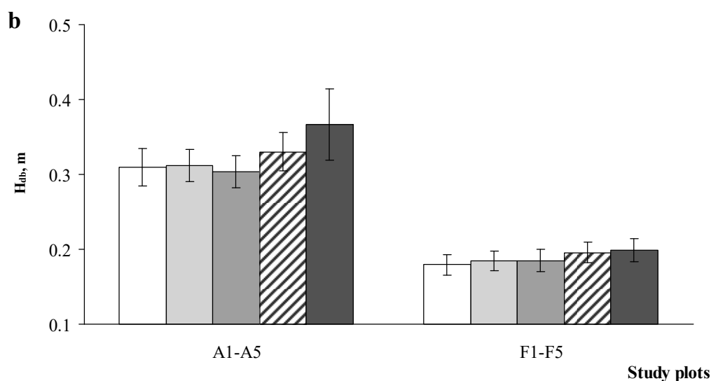
Figure 3. Mean height of the lowest live branch ( H_{lb} ) (a) and height of the lowest dead branch ( H_{db} ) (b) in two Scots pine study sites (study plots A1–A5 and F1–F5). Bars show standard error of the mean. Different capital letters A, B and C given at the top of the column show statistically significant differences between the sites at p < 0.05 ; no letters indicate no significant differences.
