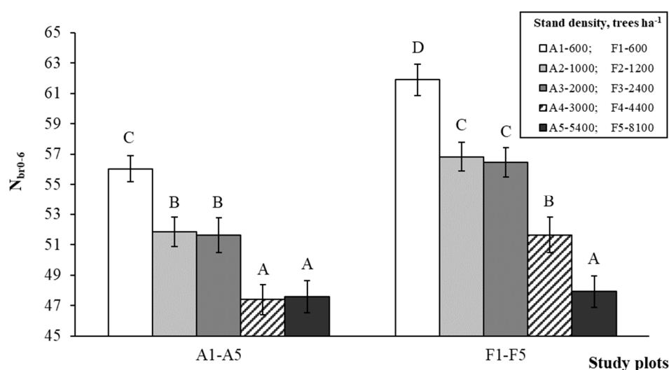
Figure 2. Mean number of branches in 0–6-m log, N_{br0-6} in two Scots pine study sites (study plots A1–A5 and F1–F5). Bars show standard error of the mean. Different capital letters A, B, C and D given at the top of the column show statistically significant differences between the sites at p < 0.05 .
