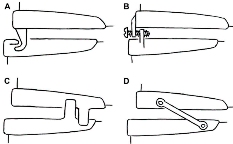
Figure 1. Schematic overview of titratable, duobloc mandibular advancement device (MAD) designs used in current clinical practice: (A) MAD with an anteriorly articulating component that allows the MAD for adjustment of the appliance; (B) MAD with attachments for the adjustment of mandibular protrusion in the frontal teeth area; (C) MAD with two lateral positioning attachments that permit incremental protrusion of the mandible; (D) MAD with lateral telescopic rods that force the mandible into an anterior position. (Figure published in Dieltjens et al., 2012 [31]).
