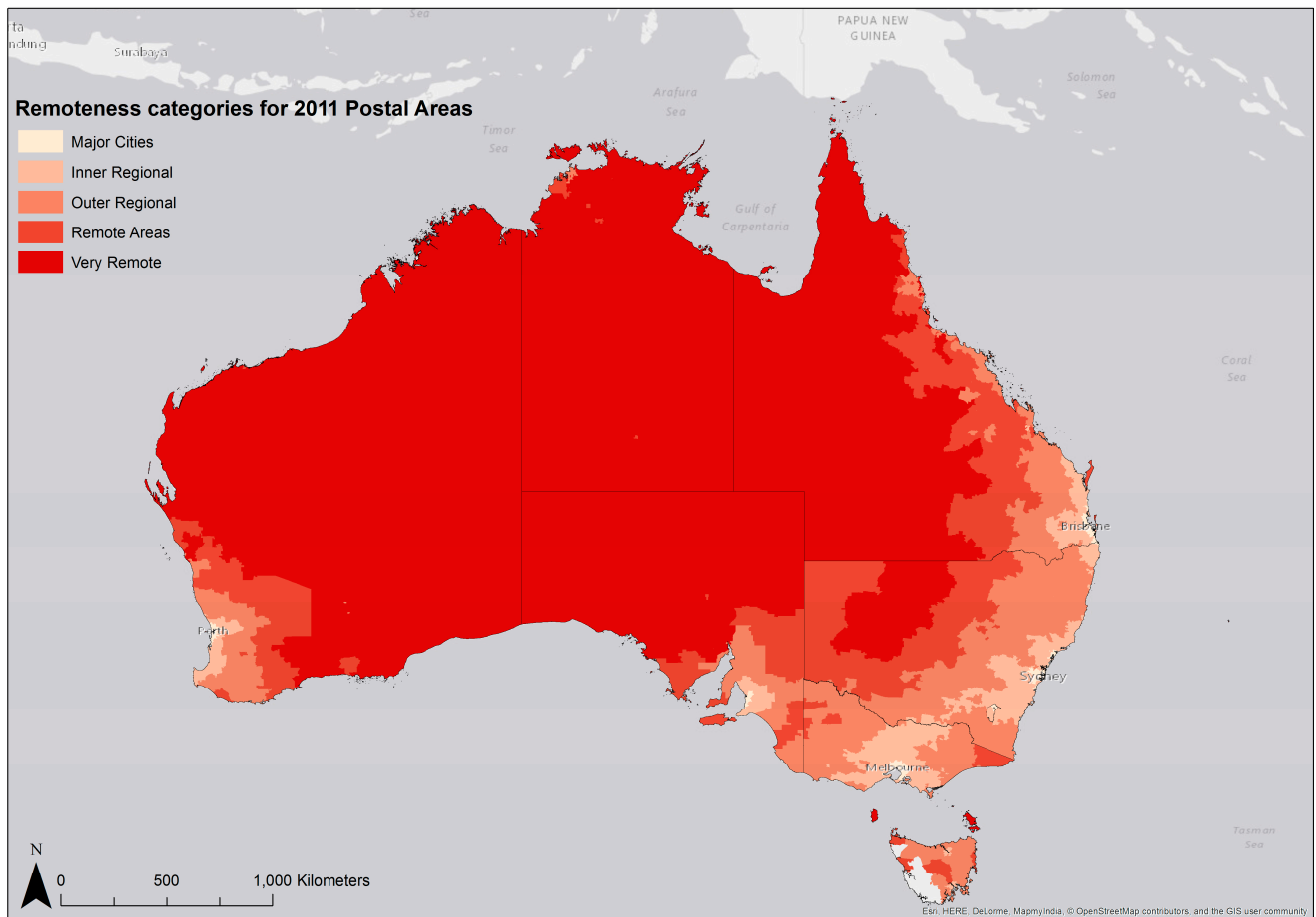
Figure S1. Remoteness categories by 2011 Postal Areas across Australia.
