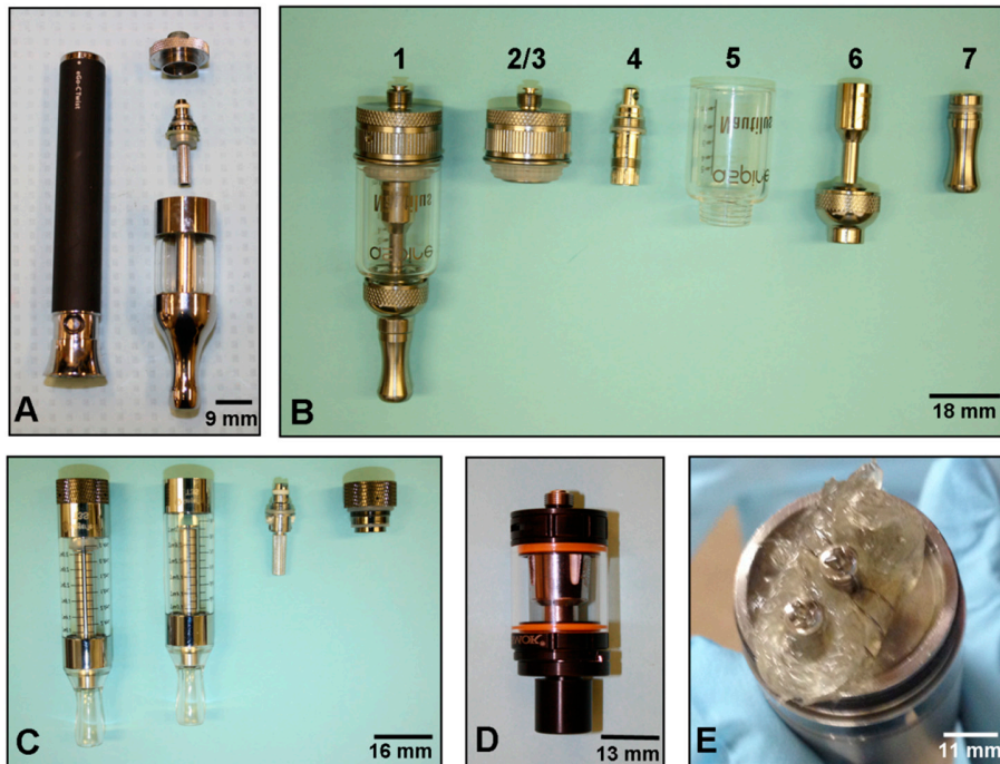
Figure S2. Anatomy of various tank style EC. A. Disassembled Kangertech Protank with associated coil and bottom hardware. B. Disassembled Aspire Nautilus tank and associated components: 1= fully assembled Aspire tank, 2/3 = bottom hardware and air-flow adjustment ring, 4 = replaceable atomizer/coil, 5 = Pyrex glass tank, 6 = upper hardware, 7 = drip tip/ mouthpiece. C. Disassembled Kanger T3S tank with associated coil and bottom hardware. D. Detail of fully assembled Smok tank. E. Anatomy of an unused Clone atomizer saturated with refill fluid.
