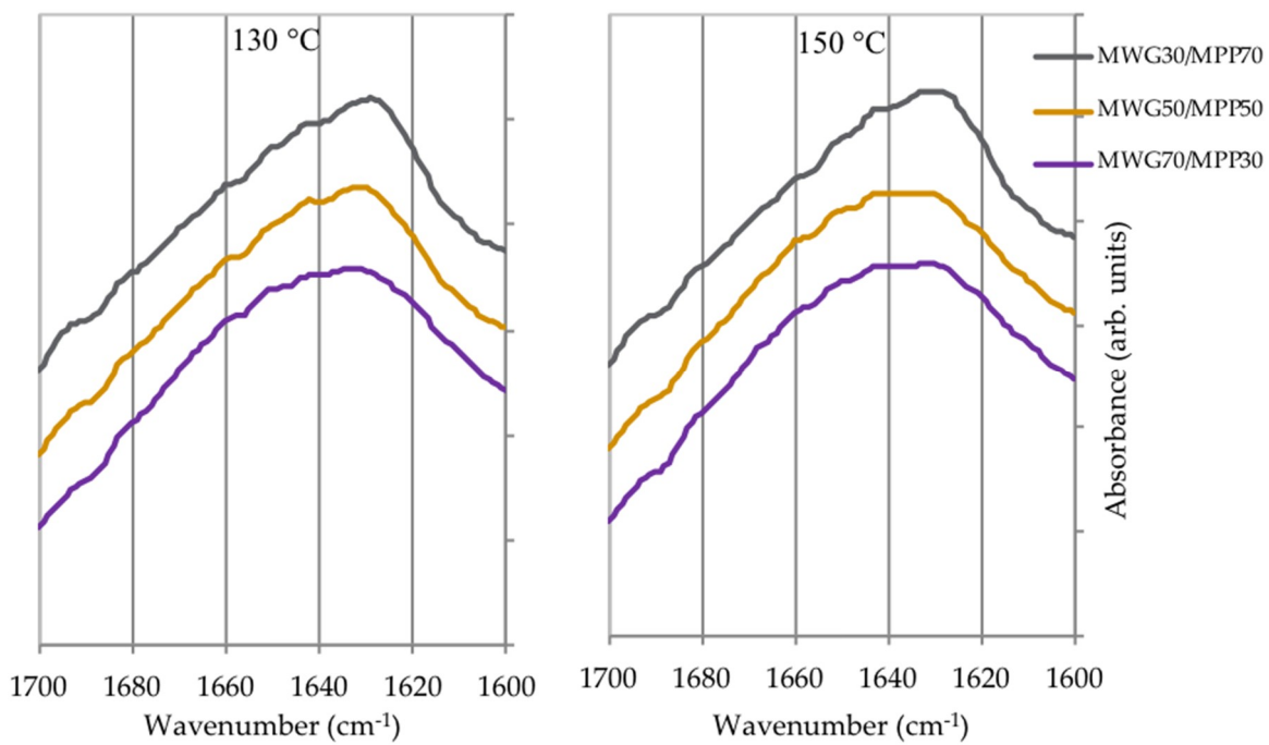
Figure S3. FT-IR spectra of MWG/MPP blends, one pressed at 130 and another one at 150 °C.
