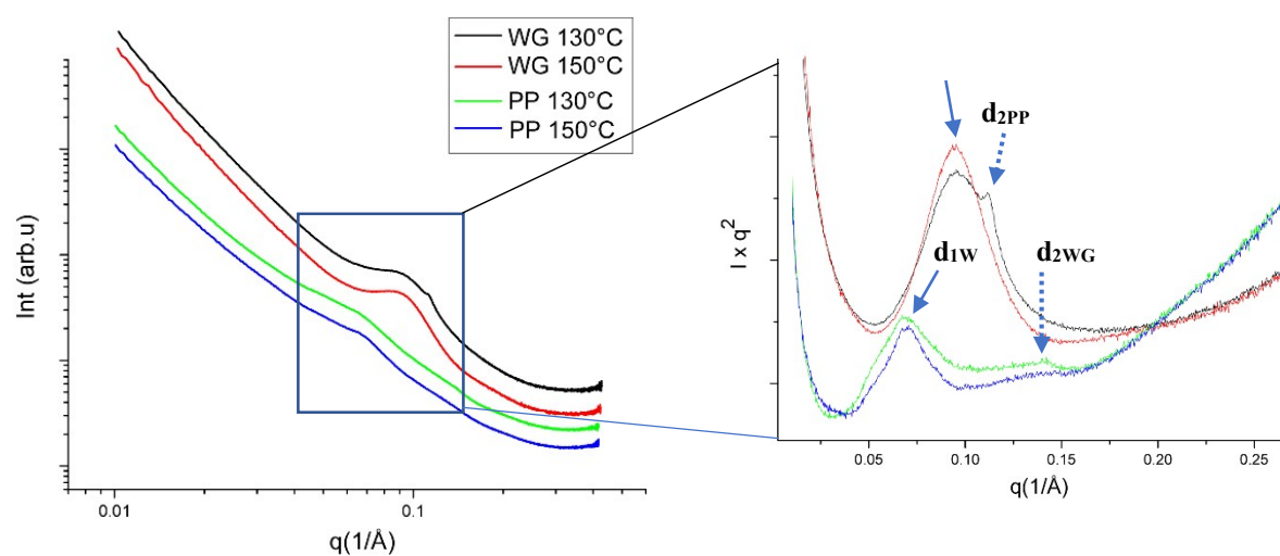
Figure S1. SAXS curves of WG and PP pressed one at 130 and another one at 150 °C. Curves are shifted vertically for clarity and I \times q^2 plot is drawn to enhance the behavior of d_1 and d_2 peaks.
