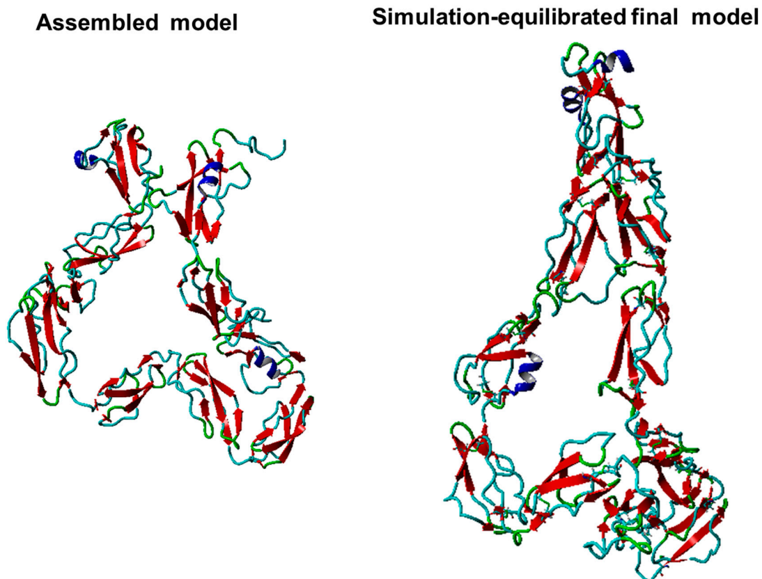
Figure S2. Difference in structures of the assembled model and the simulation equilibrated final model.
