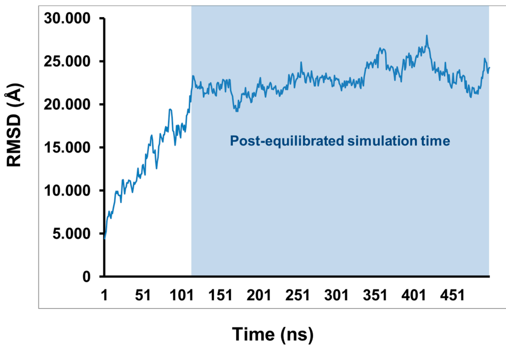
Figure S1. The RMSD graph for MD simulation-equilibration run of the FXIII-B subunit model. The region under blue shade is the production phase representing post equilibration simulation run.
