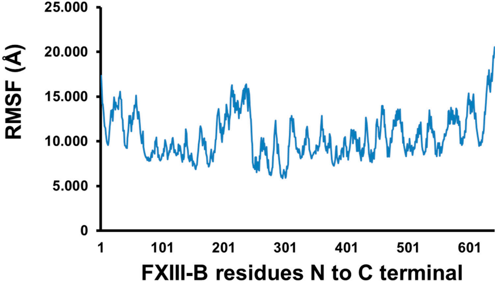
Figure S3. Flexibility/ RMSF graph for the FXIII-B subunit monomer model simulation.
