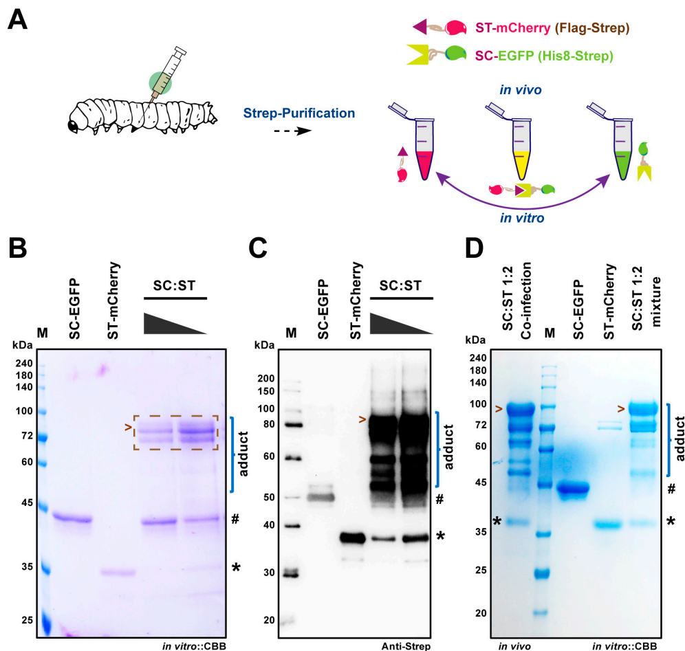
Figure 3. In vitro and in vivo protein ligation of ST/SC partners in silkworm-Spy-BEVS. (A) Diagram of expression and ligation of ST-mCherry and SC-EGFP proteins in silkworm-BEVS. Each protein was purified from the fat body of infected fat body and mixed in a decreased ratio of SC-EGFP/ST-mCherry (SC/ST) to investigate the in vitro ligation activity as demonstrated in (B) (CBB staining) and (C) (Western blot analysis by anti-Strep tag). The in vivo ligation was tested by co-infecting silkworm larvae with two recombinant baculoviruses of SC-EGFP and ST-mCherry (SC/ST = 1:2) together. The resulting products were purified by Strep-column and assessed by SDS-PAGE (D). # and * indicate SC-EGFP and ST-mCherry, respectively. Ligated products were marked by the brace and the completed adduct was marked by arrows.
