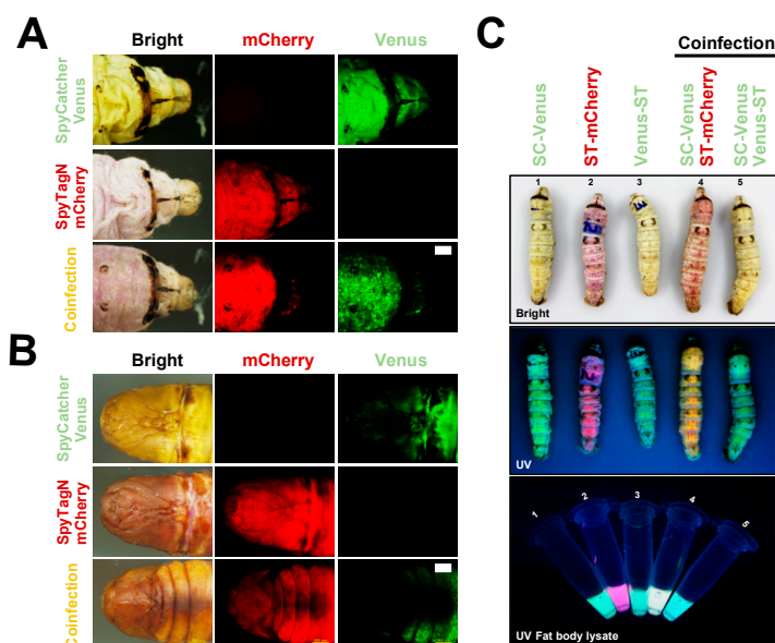
Figure 2. Production of ST- and SC-tagged proteins in silkworm-BEVS. Recombinant bacmid (s) from ST/SC constructs, SC-Venus and ST-N-mCherry were pre-mixed with DMRIE-C transfection reagents and then injected into the third day of silkworm 5th instar larvae (A) and silkworm pupae (B). The fluorescent signals of EGFP, Venus or mCherry were verified under ultraviolet light (UV). Meanwhile, the whole silkworm larvae and lysates of fat body tissue at 5 d post-infection (dpi) of recombinant baculoviruses were also investigated for fluorescent signals (C: upper panel, larvae body under bright light; middle panel, larvae body under UV light; fat body lysates under UV light). All the corresponding expressions could be verified based on the colors of the epidermis or the crude lysate of fat body tissue.
