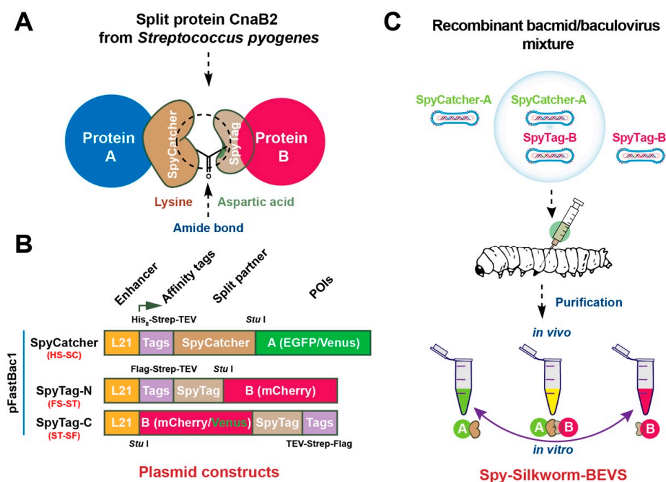
Figure 1. Schematic design of SpyTag/SpyCatcher-Bacmid/Baculovirus expression vector system (SpyBEVS). (A) Lysin-Aspartic acid amide bond formation between SpyTag/SpyCatcher-fused (ST/SC) partners. (B) Expression (pFastBac1) constructions of SpyCatcher and SpyTag (N/C-terminus). L21, a 5' untranslated leader sequence (21 bp) from a lobster tropomyosin cDNA as an enhancer to improve the protein expression level in BEVS [31]; His 8 , 8 × histidine tag; Strep, Strep-tag; TEV, a recognition site of TEV protease; FLAG, DYKDDDDK-tag. GGGG linker is presented between each tag to increase the plasticity of whole proteins. As shown, enhanced green fluorescent protein (EGFP), Venus, or mCherry proteins were employed as model proteins for each construct to be investigated in the ligation assay. (C) The experimental flow of Spy-Silkworm-BEVS using silkworm instar larvae. Recombinant baculoviruses containing ST/SC-fused proteins of interest were generated by Bac-to-Bac system. The silkworm 5th instar larvae were then injected with single or mixed recombinant bacmids or recombinant baculoviruses to produce ST/SC-fused proteins for in vitro (after protein purification) and in vivo (co-expression in silkworm via co-infection methods) ligation, respectively.
