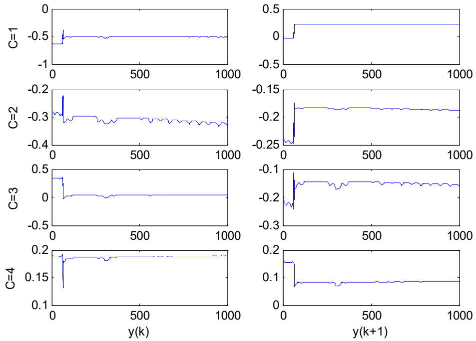
Figure 10. Center curve of the Gaussian membership function.
