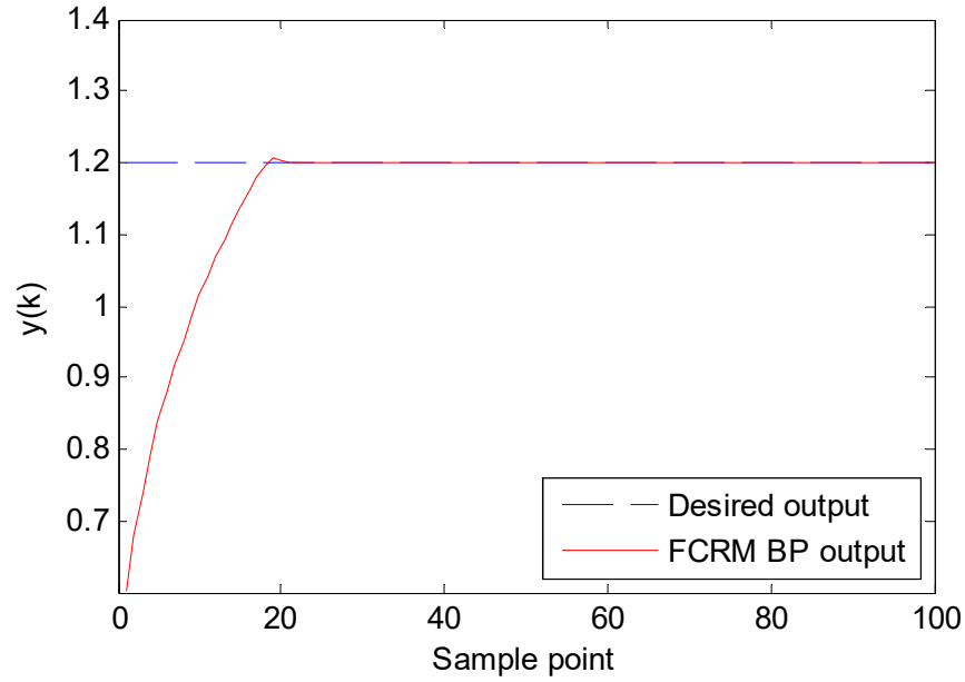
Figure 15. Proposed method and desired output curve.
