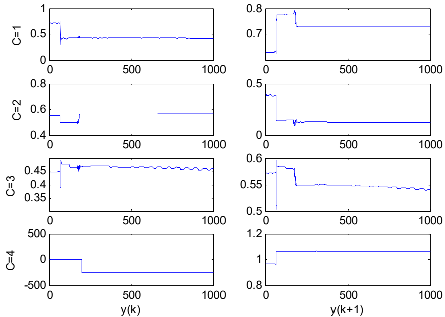
Figure 11. Width curve of the Gaussian membership function.
