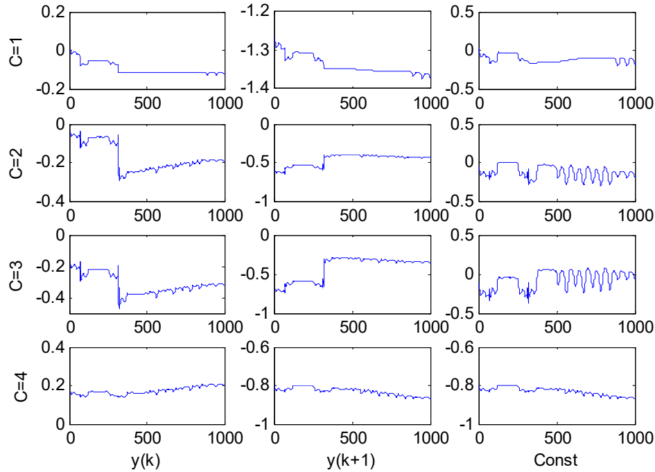
Figure 12. Consequent parameter curve of the T-S fuzzy model.
