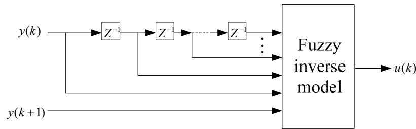
Figure 1. Fuzzy inverse modeling structure.
