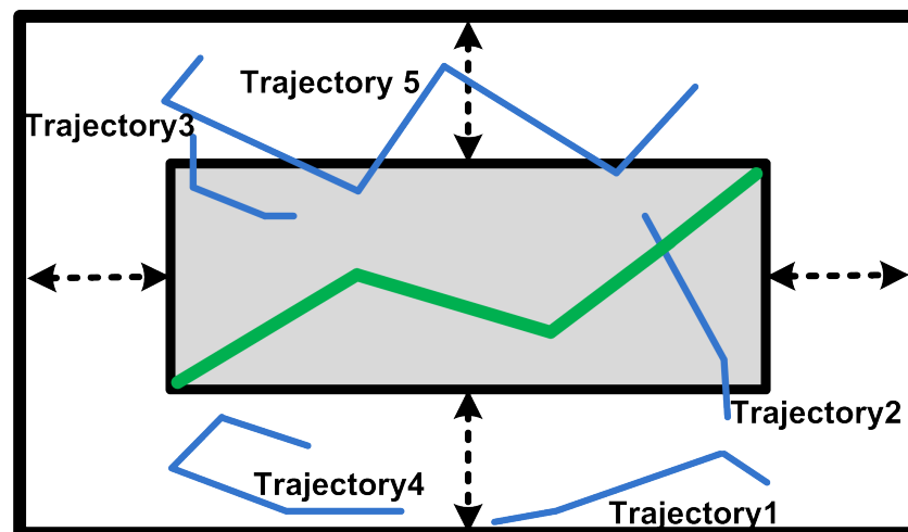
Figure 2. Overlapped trajectories.
