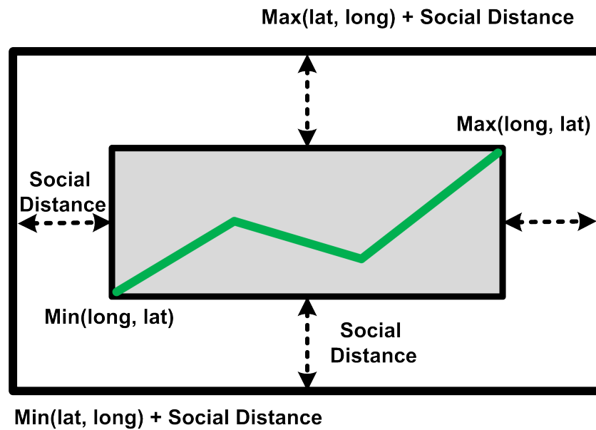
Figure 1. Overlapped region.
