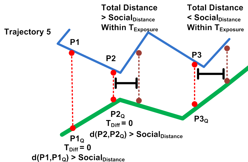
Figure 3. Computing exposure.
