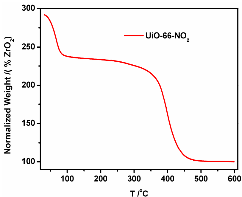
Figure S2. TGA plot of UiO-66-NO 2 under air flow based on the normalization of ZrO 2 to 100%. The defect amount is estimated based on the normalized weight at 350 °C.
