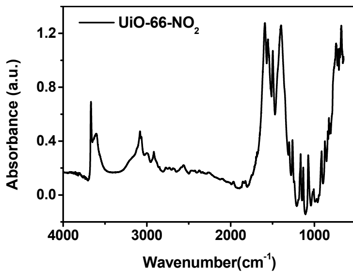
Figure S3. DRIFTS spectrum of UiO-66-NO 2 .
