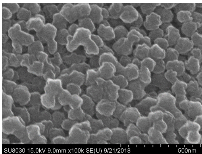
Figure S1. A SEM image of UiO-66-NO 2 .
