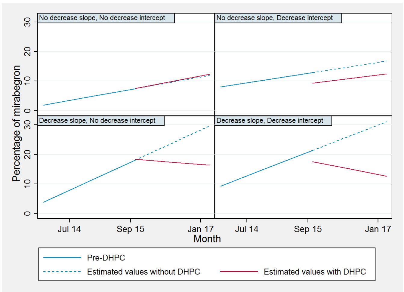
Figure S1. Estimated values for proportion of mirabegron prescribing with and without the direct healthcare professional communication (DHPC), graphed by significant reduction in slope or level post-DHPC.
