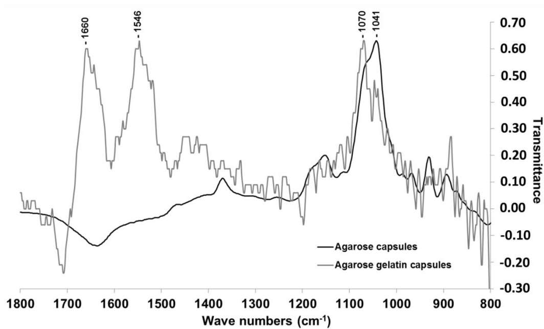
Figure S1. FTIR spectra of agarose microcapsules and agarose-gelatin microcapsules.
