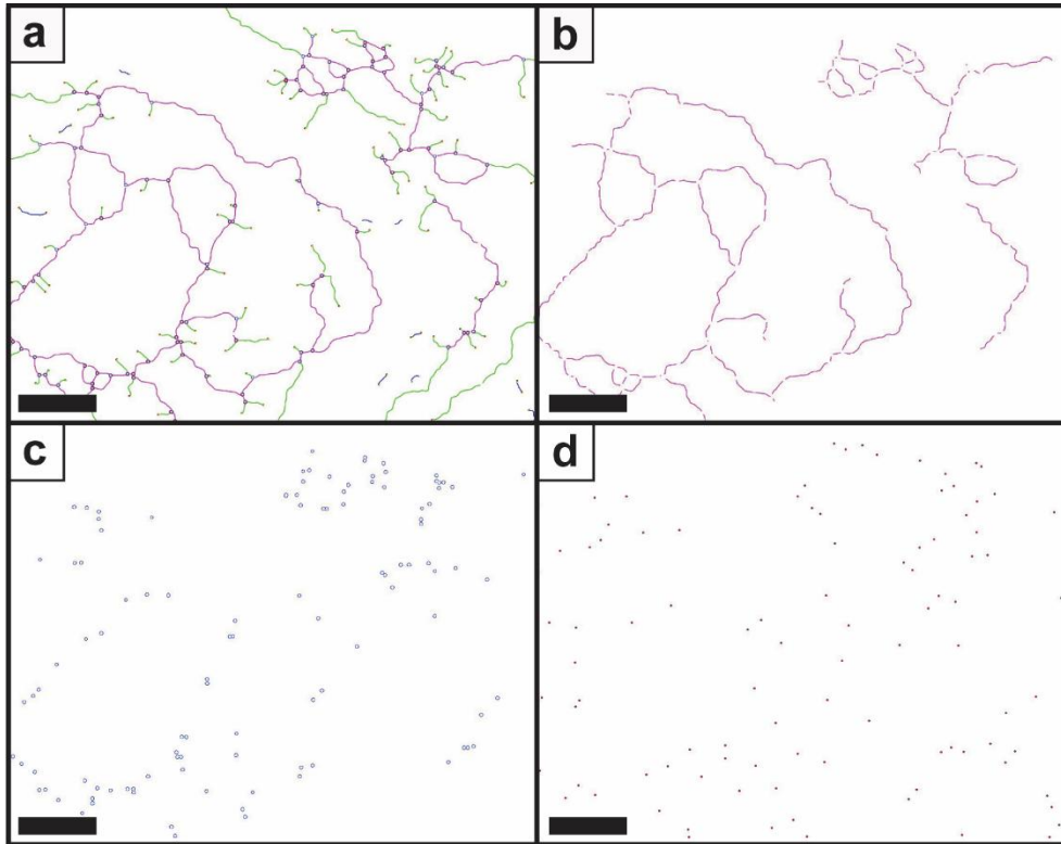
Figure S1. Selection and display of single elements after the image processing. The plug-in Angiogenesis Analyzer allows the feature identification and display starting from (a) the structure analysis; to (b) the node to node struts which are shown in purple; (c) the number of nodes; and (d) the number of termini. Scale bars represent 100 \mu\text{m} .
