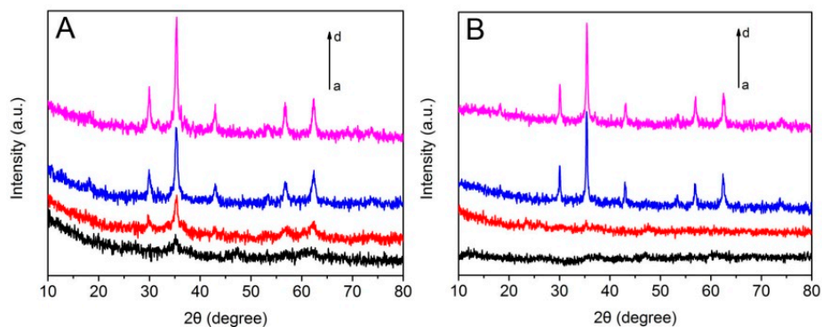
Figure S1. XRD patterns of the intermediates prepared from (A) the hollow \text{ZnFe}_2\text{O}_4 ; and (B) solid \text{ZnFe}_2\text{O}_4 systems: (a) 0.5 h, (b) 1 h, (c) 2 h, and (d) 4 h.
