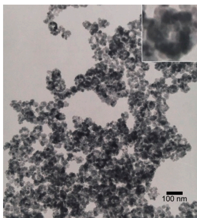
Figure S2. TEM image of \text{ZnFe}_2\text{O}_4 CNAs when the volume ethylene glycol/ethanol ratio (EG/Et) in the solvent is 1:8.
