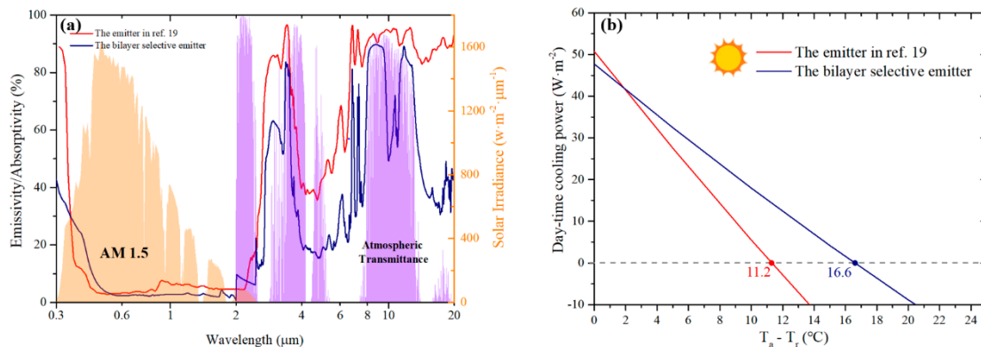
Figure S1. the comparison of (a) the solar and IR emissivity/absorptivity and (b) the day-time cooling power between between the bilayer selective emitter and a selective emitter in ref. [19].
