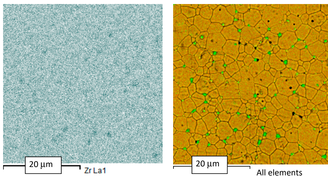
Figure S1. SEM image and EDX mapping of the elements on the surface of SZY0.94 after polishing and thermal etching at 1400 °C.
