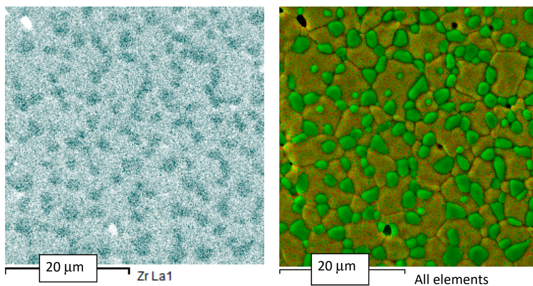
Figure S2. SEM image and EDX mapping of the elements on the surface of SZY0.94 after polishing and thermal etching at 1650 °C.
