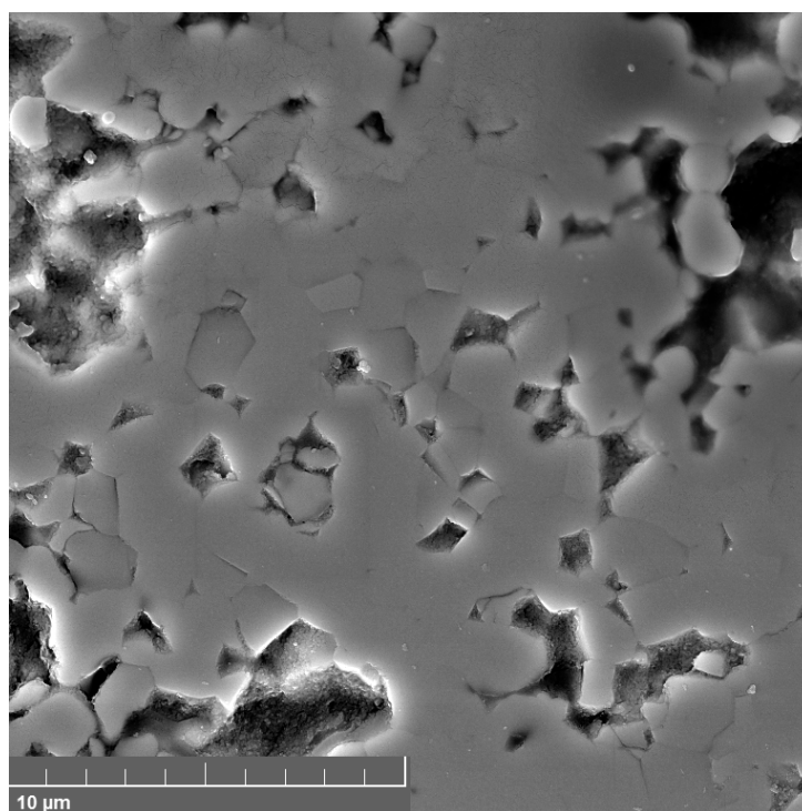
Figure S3. SEM image of as-polished cross-section of SZY1.00.
