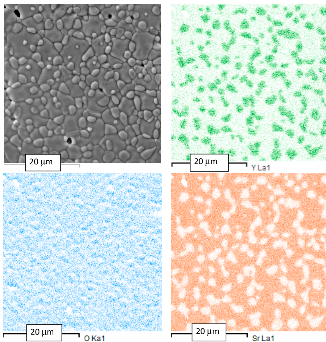
Figure S1. SEM image and EDX mapping of the elements on the surface of SZY0.94 after polishing and thermal etching at 1400 °C.
