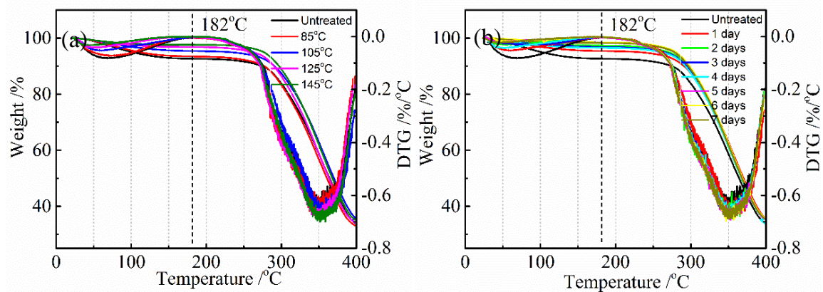
Figure S1. TGA curves and DTG curves of collagen films with DHT treatment, (a) at various DHT temperatures for 1 day; (b) for various DHT time at 105 °C.
