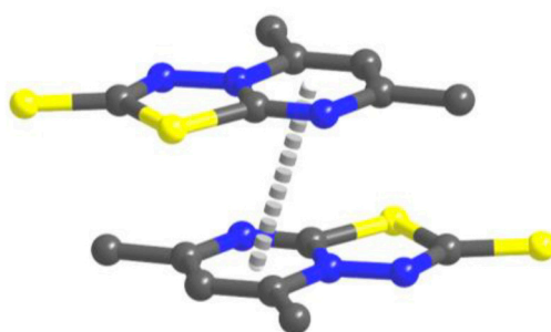
Figure S1. Supramolecular dimer of (1) in the solid state.
