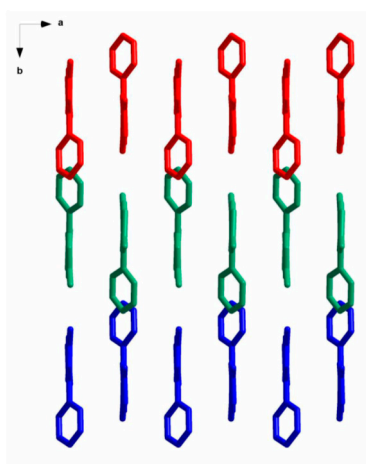
Figure S2. Crystal packing of (2) in the ab plane.
