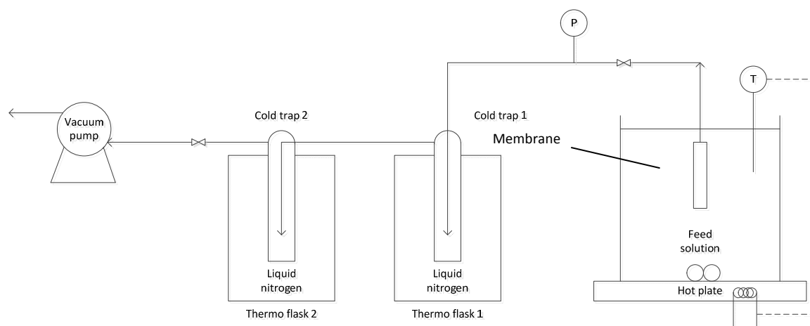
Figure 1. Experimental setup.
