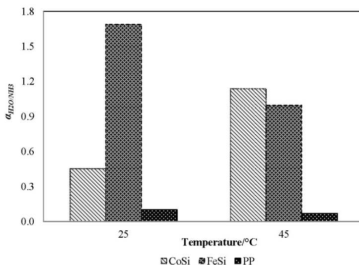
Figure 4. The water/ammonia separation factor, \alpha_{H_2O/NH_3} , of the CoSi and FeSi membranes at different feed temperature (synthetic solution of 1000 mg/L ammonia concentration; permeate absolute pressure, 100–150 Pa).
