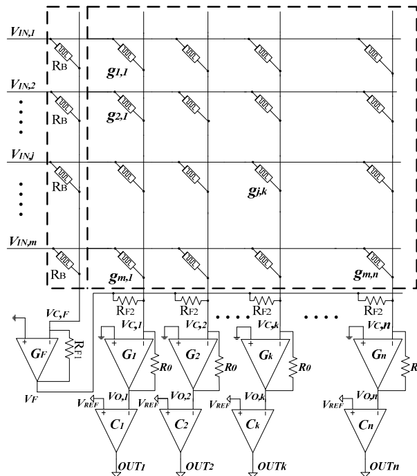
Figure 1. The memristor-based crossbar architecture with a single memristor array and a constant-term circuit for realizing the synaptic matrix of a perceptron neural network [21].
