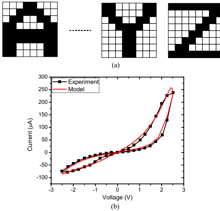
Figure 5. (a) The eight \times eight pixels images of characters used to test the proposed memristor crossbar circuit. (b) The memristor’s current–voltage characteristic measured from the real device and the memristor’s behavior model [28,29].
