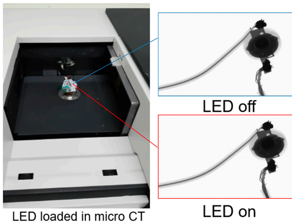
Figure S1. X-ray stability and recognition of the micro-IR LED with a micro-CT machine.
