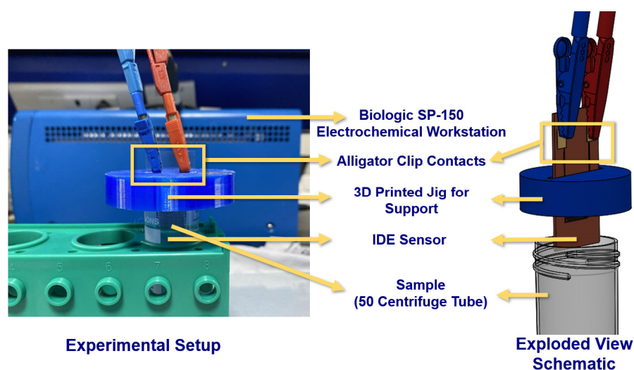
Figure 3. Experimental setup and schematic showing the enhanced view of the experimental setup for EIS analysis using potentiostat. A two-electrode configuration was employed with a frequency ranging from 1 Hz to 1 MHz.
