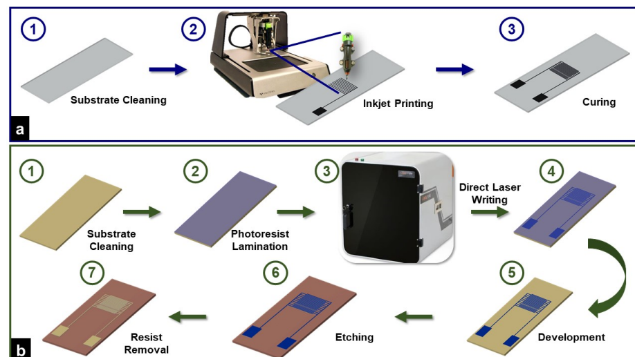
Figure 2. Overall step-by-step fabrication scheme for (a) Carbon ink-based IDE printed on glass slide (b) Photolithography-based DLW IDE on a copper-cladded FR4 PCB board.
