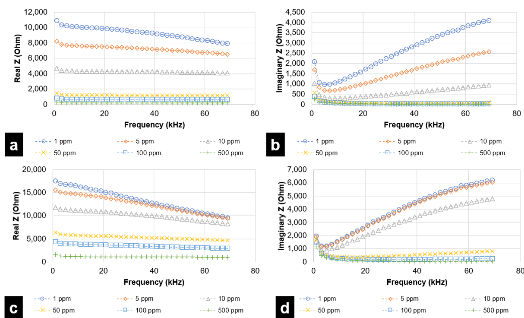
Figure 9. EIS analysis for Citric Acid (sour) and L-tryptophan (bitter), in the range of 1 kHz to 69 kHz, for DLW-photolithography-based IDE sensor in terms of (a) Resistive Impedance vs. Frequency (Citric Acid) (b) Reactive Impedance vs. Frequency (Citric Acid) (c) Resistive Impedance vs. Frequency (L-tryptophan) (d) Reactive Impedance vs. Frequency (L-tryptophan).
