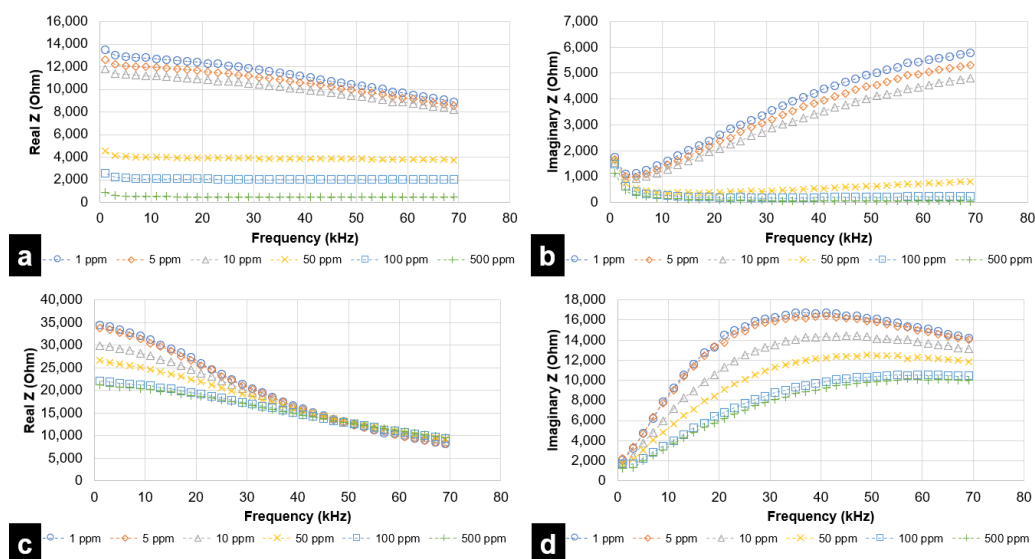
Figure 10. EIS analysis for GMP (umami) and sucrose (sweet), in the range of 1 kHz to 69 kHz, for DLW-photolithography-based IDE sensor in terms of (a) Resistive Impedance vs. Frequency (GMP) (b) Reactive Impedance vs. Frequency (GMP) (c) Resistive Impedance vs. Frequency (sucrose) (d) Reactive Impedance vs. Frequency (sucrose).
