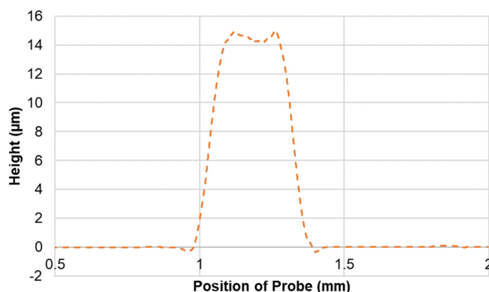
Figure 5. Profile obtained for thickness of single finger of inkjet printing-based (IDE) sensor measured using a stylus profiler.
