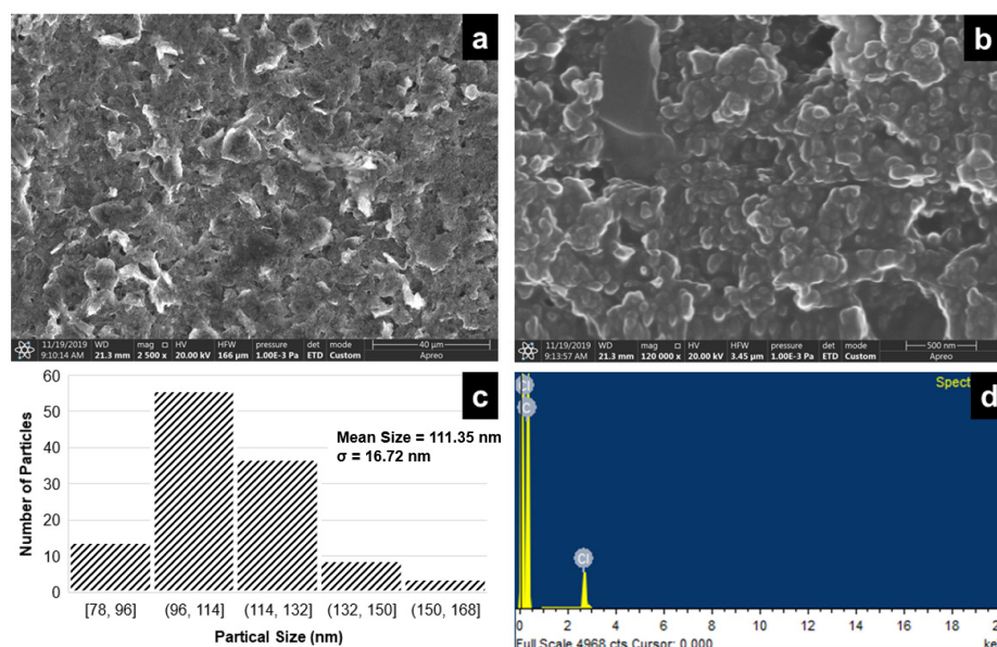
Figure 4. SEM image of inkjet-printed carbon ink at a magnification scale corresponding to (a) 40 \mu\text{m} , (b) 500 nm, (c) particle size distribution plot (mean particle size = 111.35 nm and standard deviation, \sigma = 16.72 nm) and (d) EDX analysis.
