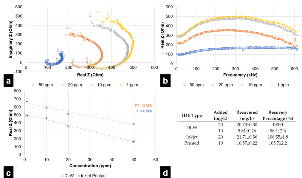
Figure 6. (a) Nyquist plot for nitrite sensing using the DLW-photolithography-based IDE sensor for different concentrations (b) real part of impedance vs. frequency plot for DLW-photolithography-based IDE sensor showing the nature of resistive impedance maximizing at 265 kHz (c) results derived from EIS analysis for nitrite concentration evaluation using inkjet printing-based IDE Sensor and DLW-photolithography-based IDE sensor in terms of resistive impedance vs concentration (d) results for the analysis of tap water for detection via recovery of nitrite at different concentrations.
