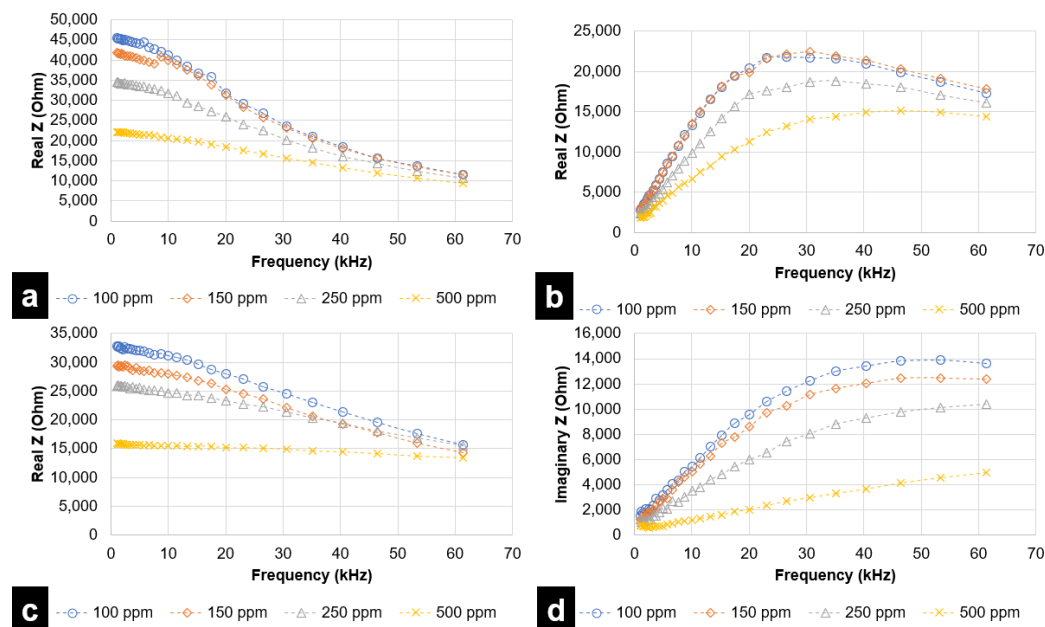
Figure 8. EIS analysis for GMP (umami) and sucrose (sweet), in the range of 1 kHz to 62 kHz, for inkjet printing-based IDE sensor in terms of (a) Resistive Impedance vs. Frequency (GMP) (b) Reactive Impedance vs. Frequency (GMP) (c) Resistive Impedance vs. Frequency (sucrose) (d) Reactive Impedance vs. Frequency (sucrose).
