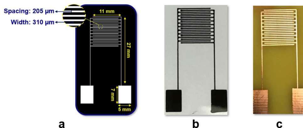
Figure 1. (a) Optimized Design (b) Carbon ink-based IDE printed on glass slide (c) Photolithography-based DLW IDE on a copper-cladded FR4 board.
