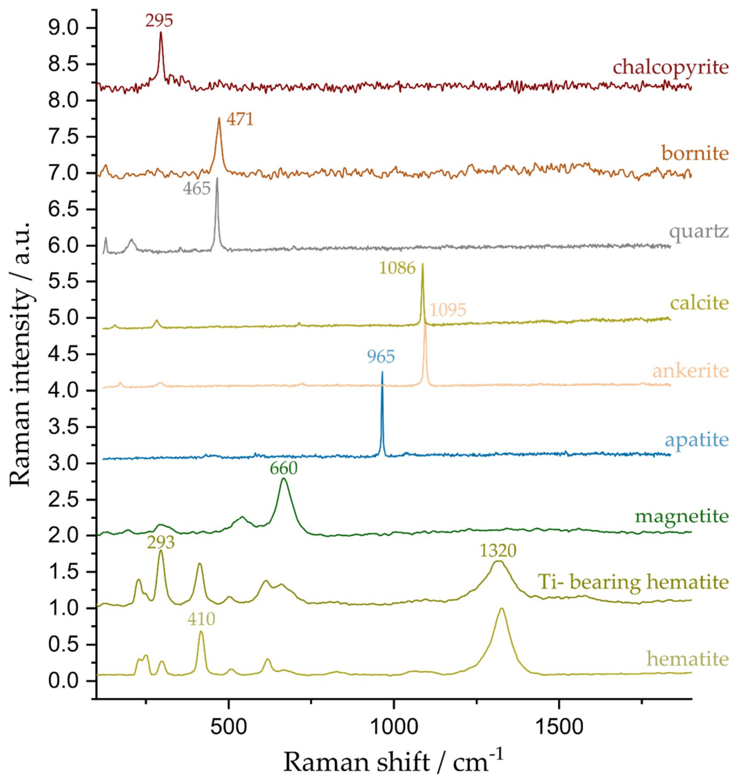
Figure S1. Reference Raman spectra. Background-corrected and normalized Raman reference spectra used for linear combination.
