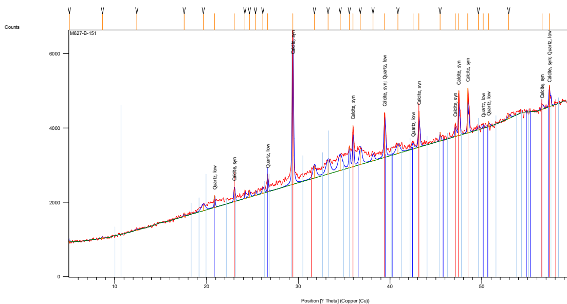
Figure S1. XRD-pattern (and identified mineral phases) of the sample GC-627/B-151.
