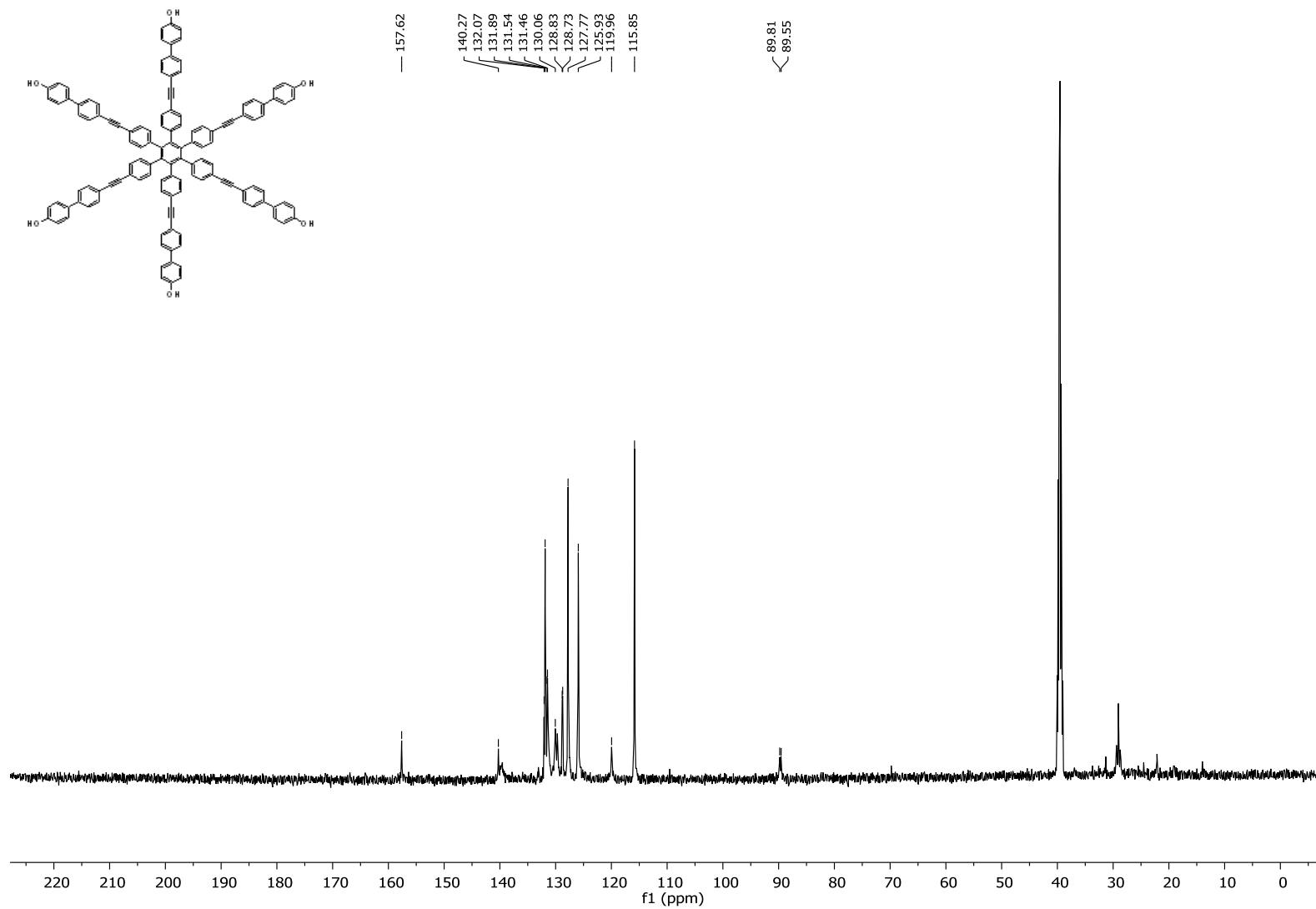
Figure S2. ^{13}\text{C} \{^1\text{H}\} (125 MHz, DMSO- d_6 ) NMR spectrum for 2.
