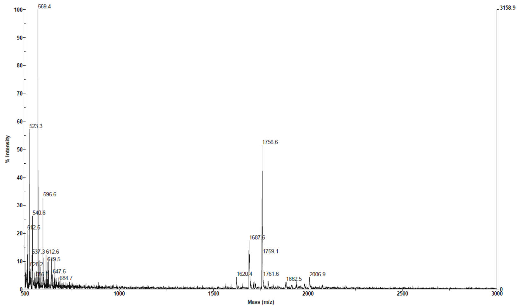
Figure S3. MALDI mass spectrum of 2.
