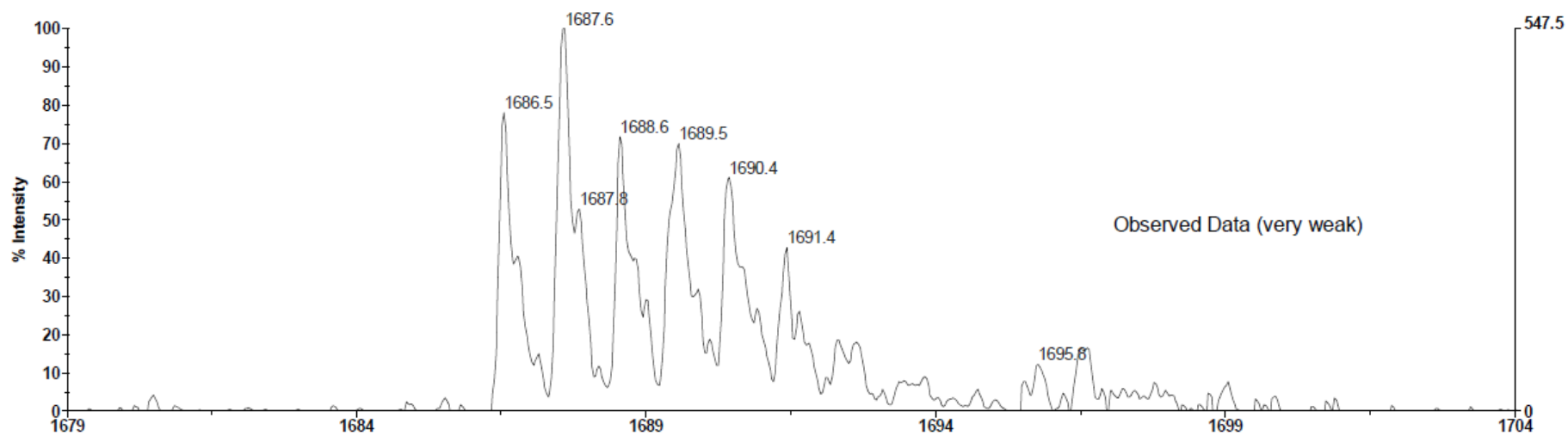
Figure S5. Observed isotope patten of 2.
