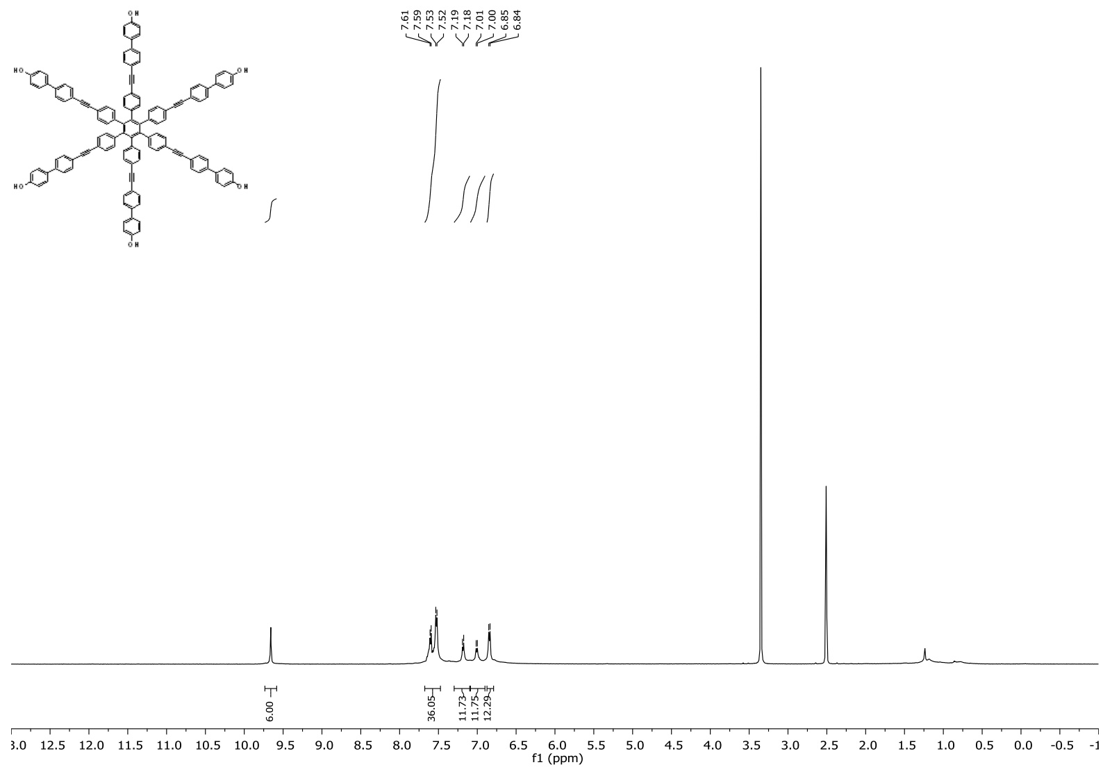
Figure S1. ^1\text{H} (500 MHz, \text{DMSO-}d_6 ) NMR spectrum for 2 .
