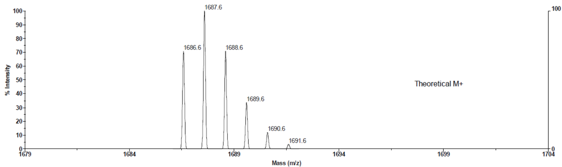
Figure S4. Theoretical isotope pattern of 2.
